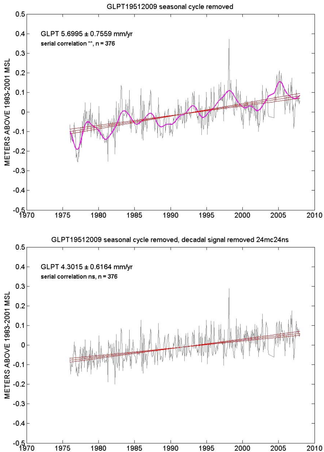
Figure B-12. RSL trends and 95% confidence intervals before (upper) and after (lower) removal of the decadal signal at GLPT, 1976-2007 period.
