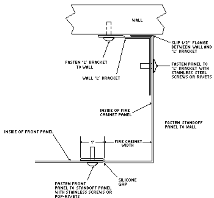
FIG. 9 FIRE CABINET PANEL
