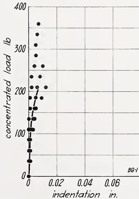
FIGURE 11.—Concentrated load on wall BG, load applied to inside face.
