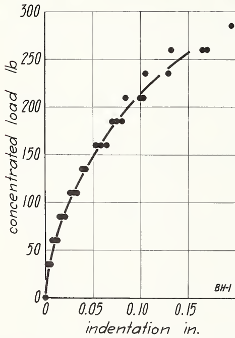
FIGURE 23.—Concentrated load on wall BH, load applied to inside face.
