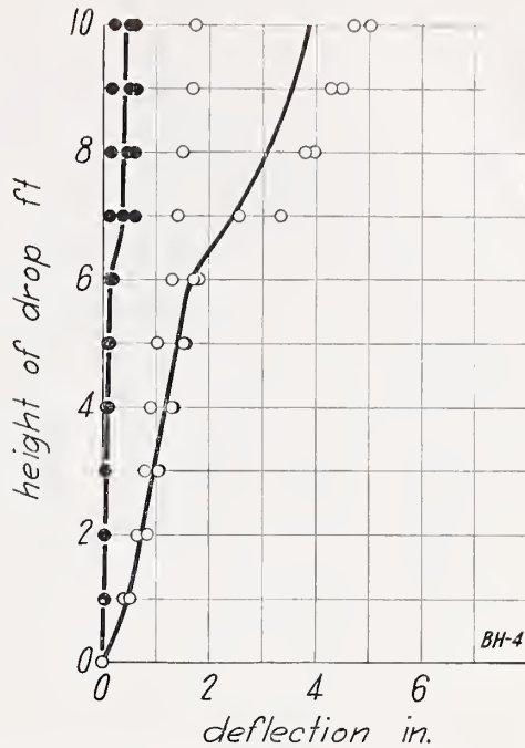
FIGURE 26.—Impact load on wall BH, load applied to outside face.
