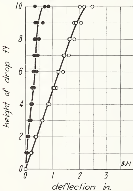
FIGURE 46.—Impact load on wall BJ , load applied to inside face.
