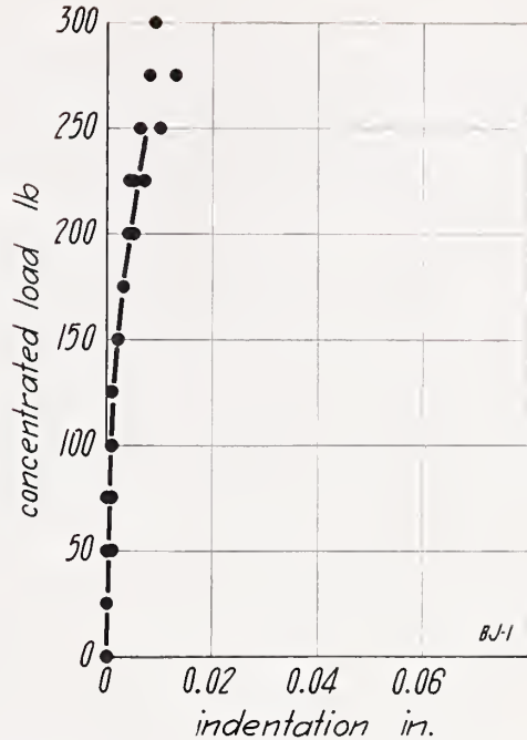
FIGURE 44.—Concentrated load on wall BJ, load applied to inside face.
