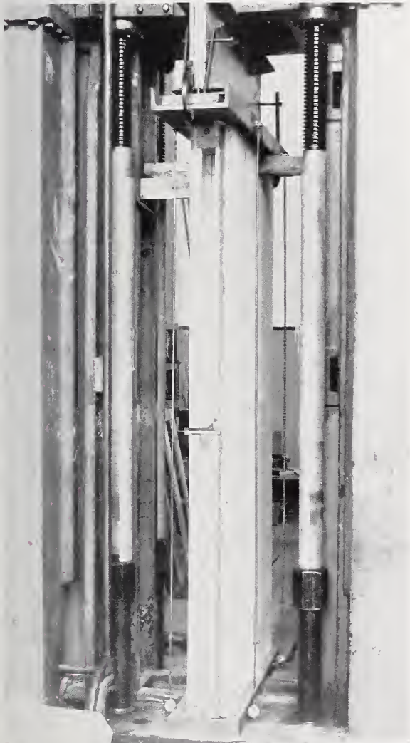
FIGURE 39.—Wall specimen BJ-C2 under compressive load.
