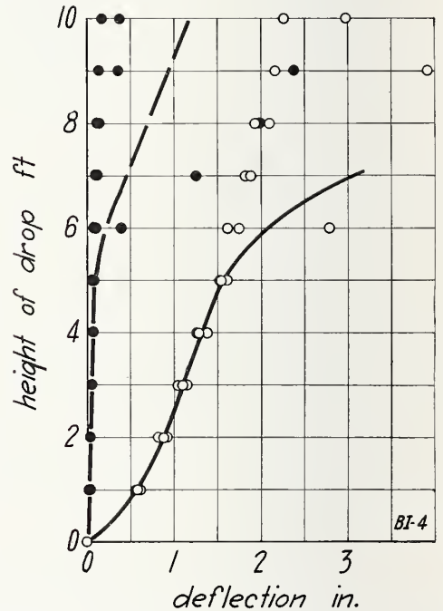
FIGURE 36.—Impact load on wall BI , load applied to outside face.
