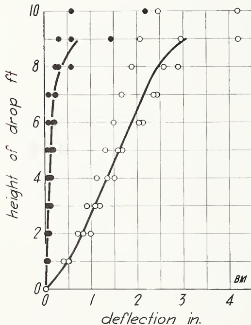
FIGURE 72.—Impact load on partition BM .
