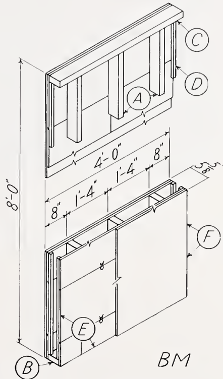
FIGURE 71.—Partition specimen BM .
