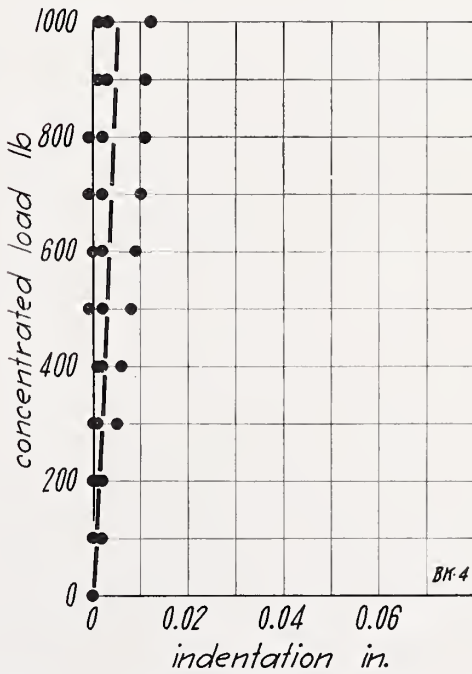
FIGURE 56.—Concentrated load on wall BK, load applied to outside face.
