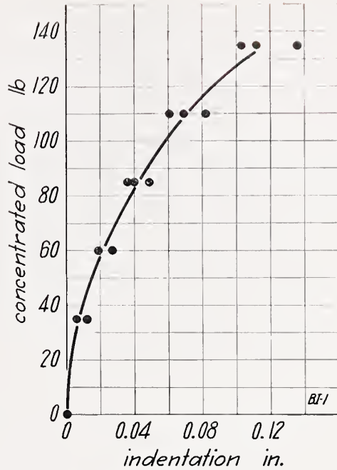
FIGURE 33.—Concentrated load on wall BI, load applied to inside face.
