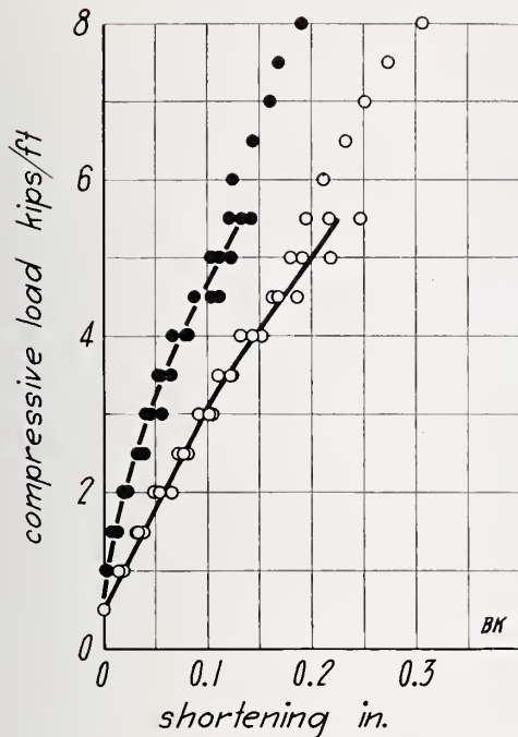
FIGURE 50.—Compressive load on wall BK.
