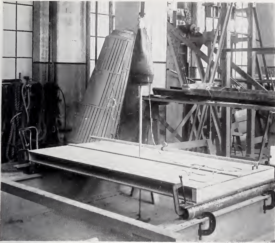
FIGURE 76.—Partition specimen BN-12 during the impact test.
