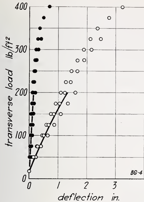
FIGURE 10—Transverse load on wall BG, load applied to outside face.
