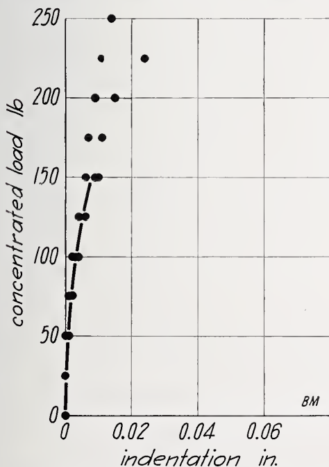
FIGURE 74.—Concentrated load on partition BM . Load-indentation results for specimens BM-P1 , P2 , and P3 .
