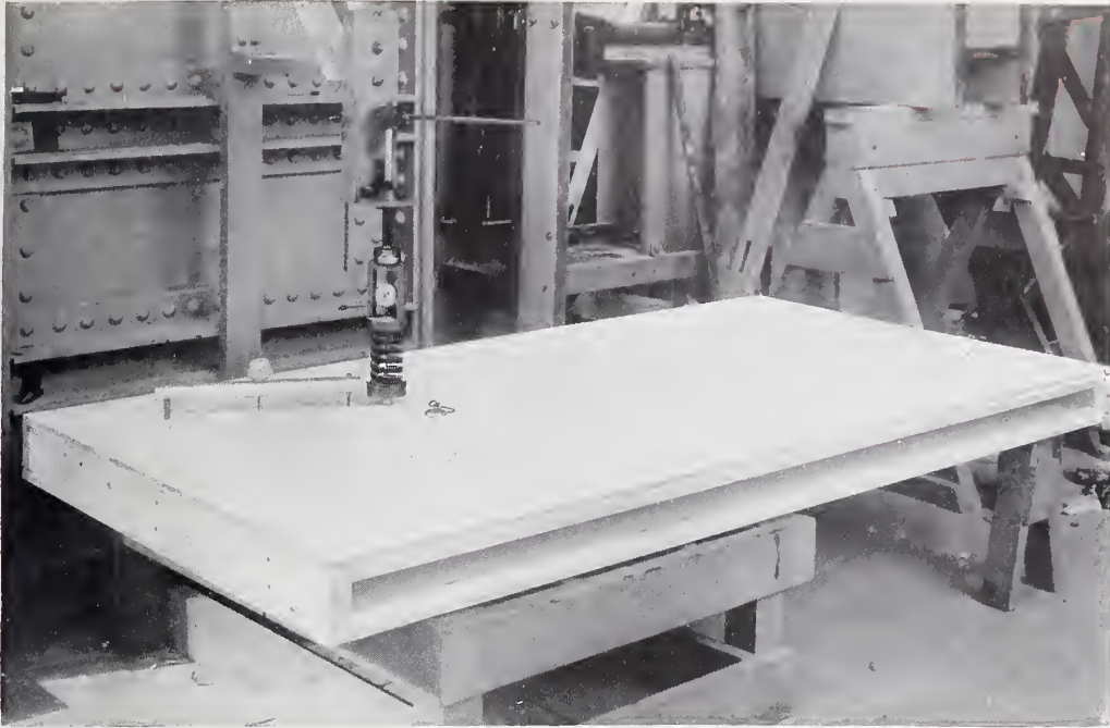
FIGURE 73.—Partition specimen BM-P2 under concentrated load.
