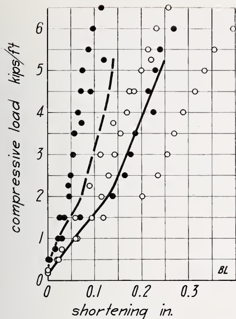
FIGURE 61.—Compressive load on wall BL.
