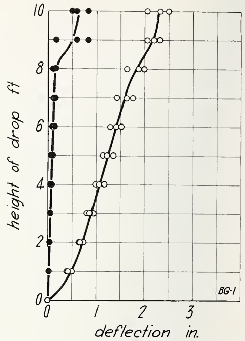
FIGURE 13.—Impact load on wall BG , load applied to inside face.
