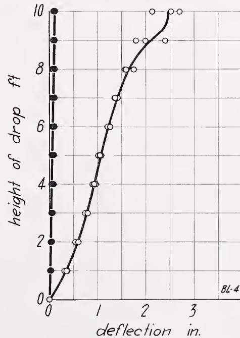
FIGURE 68. Impact load on wall BL, load applied to outside face.
