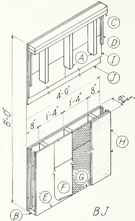
FIGURE 38.—Four-foot wall specimen BJ .
