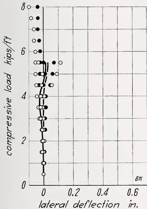
FIGURE 51.—Compressive load on wall BK.
