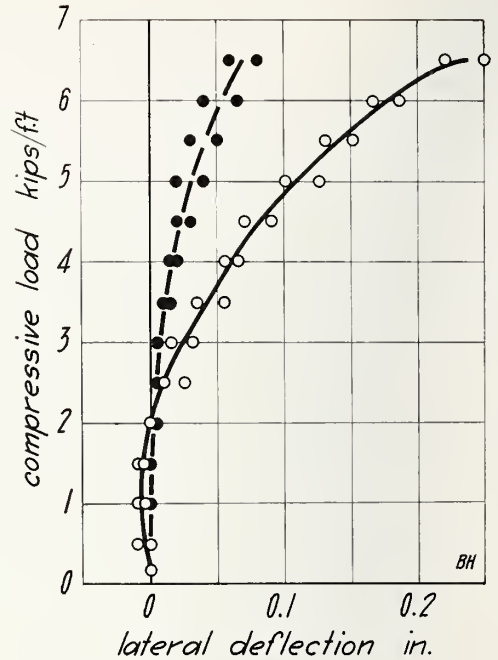
FIGURE 19.—Compressive load on wall BH .
