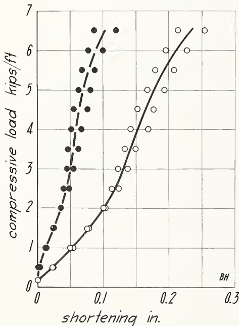
FIGURE 18.—Compressive load on wall BH .
