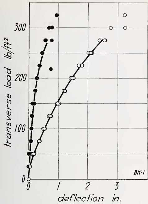
FIGURE 53.—Transverse load on wall BK, load applied to inside face.
