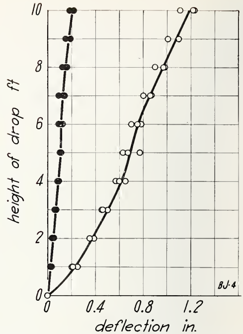
FIGURE 47.—Impact load on wall BJ , load applied to outside face.
