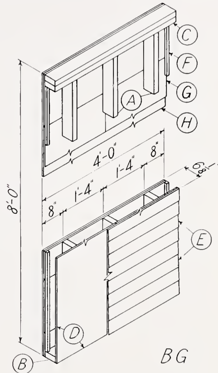
FIGURE 5.—Four-foot wall specimen BG.
