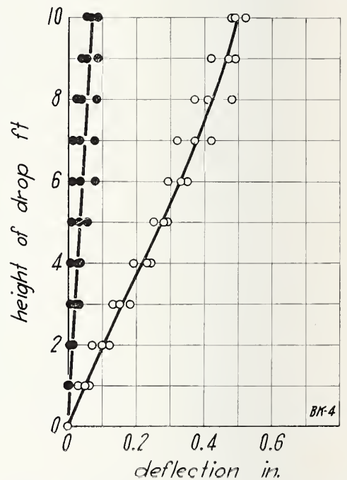
FIGURE 58.—Impact load on wall BK, load applied to outside face.
