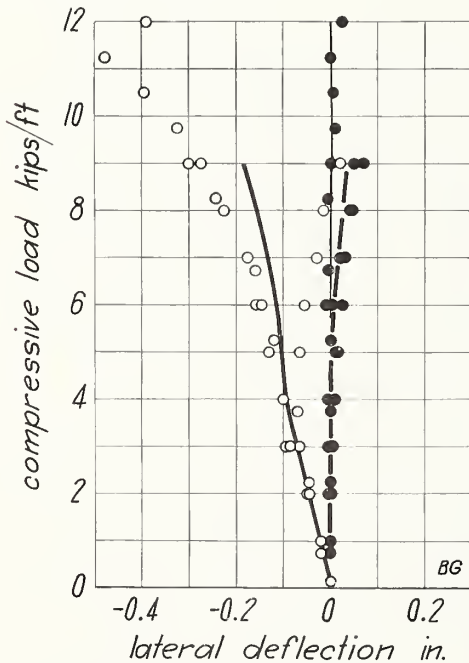
FIGURE 8.—Compressive load on wall BG.
