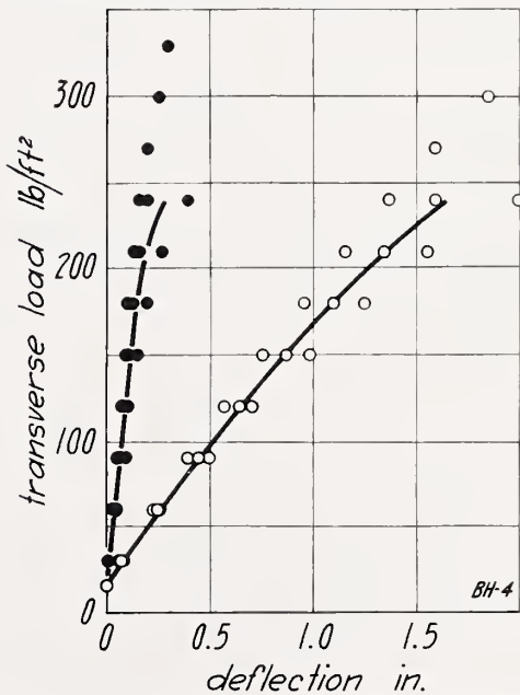
FIGURE 21.—Transverse load on wall BH-4, load applied to outside face.
