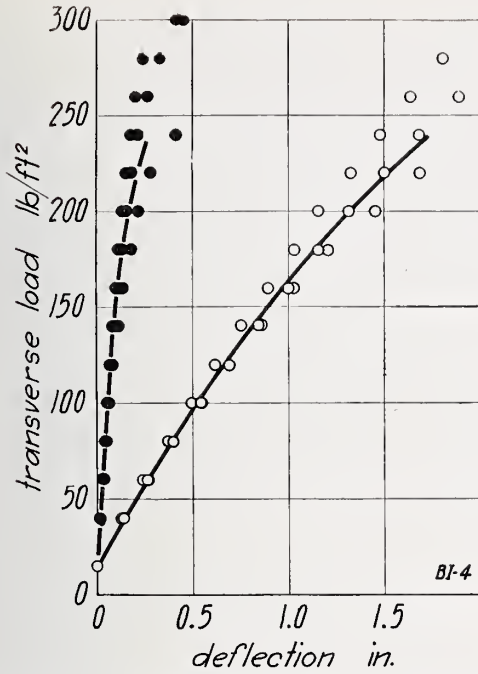
FIGURE 32.—Transverse load on wall BI, load applied to outside face.
