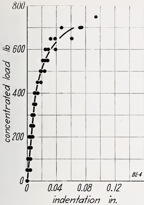
FIGURE 66.—Concentrated load on wall BL, load applied to outside face.
