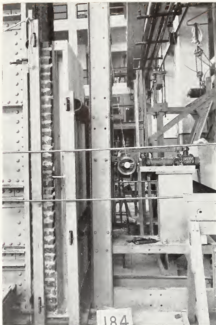
FIGURE 52.—Wall specimen BK-T3 , under transverse load.
