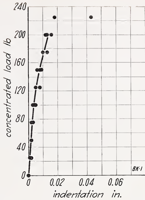
FIGURE 55.—Concentrated load on wall BK, load applied to inside face.
