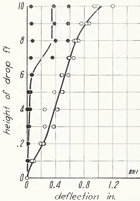
FIGURE 57.—Impact load on wall BK, load applied to inside face.
