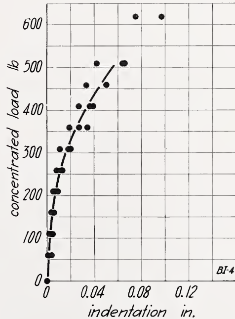
FIGURE 34.—Concentrated load on wall BI, load applied to outside face.
