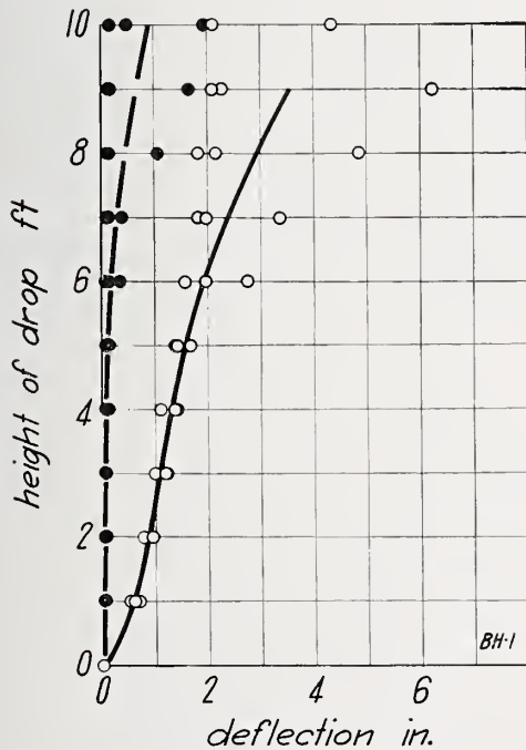
FIGURE 25.—Impact load on wall BH, load applied to inside face.
