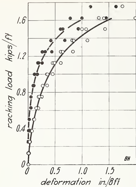
FIGURE 27.—Racking load on wall BH.
