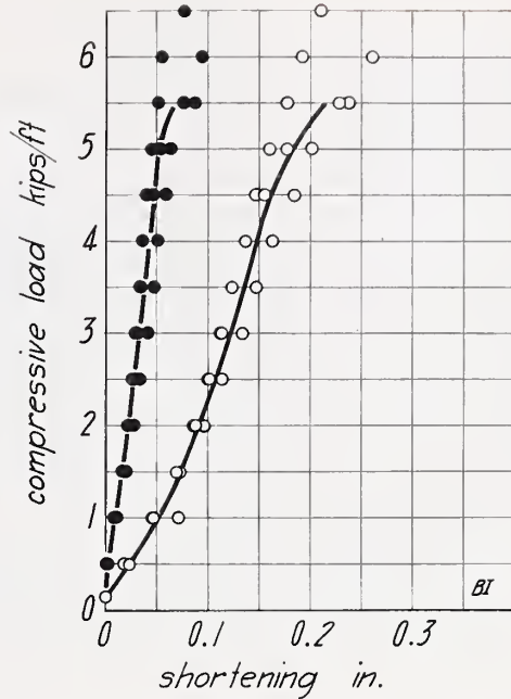
FIGURE 28.—Compressive load on wall BI .
