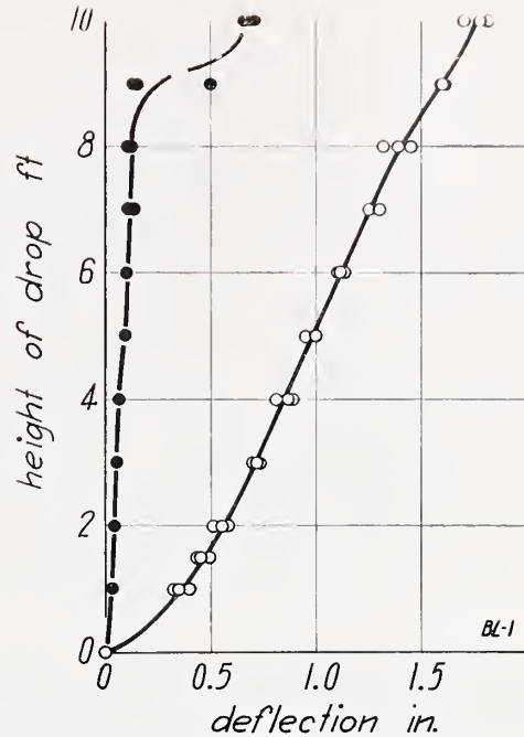
FIGURE 67.—Impact load on wall BL, load applied to inside face.
