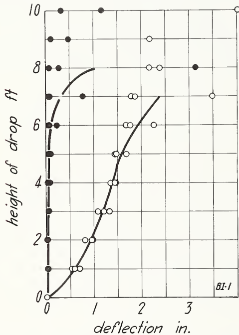
FIGURE 35.—Impact load on wall BI , load applied to inside face.
