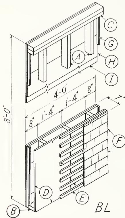
FIGURE 60.—Four-foot wall specimen BL.
