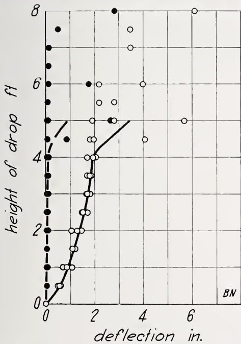
FIGURE 77.—Impact load on partition BN.
