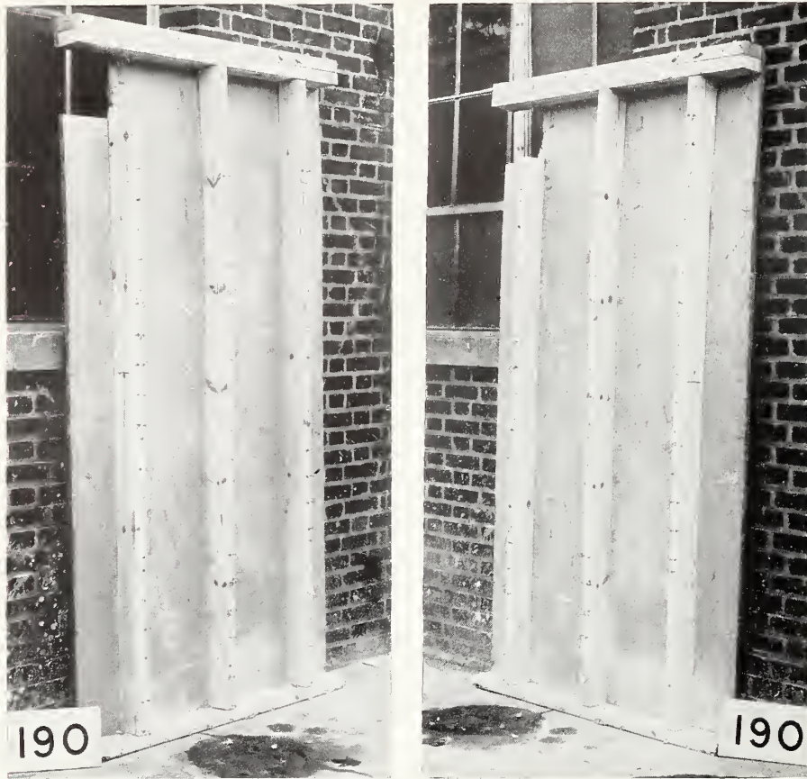
FIGURE 3.—Frame of wall specimen BK-T5.
