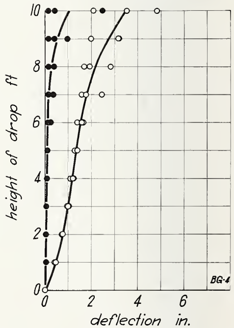
FIGURE 14.—Impact load on wall BG , load applied to outside face.
