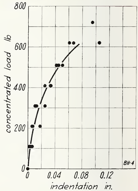
FIGURE 24.—Concentrated load on wall BH, load applied to outside face.
