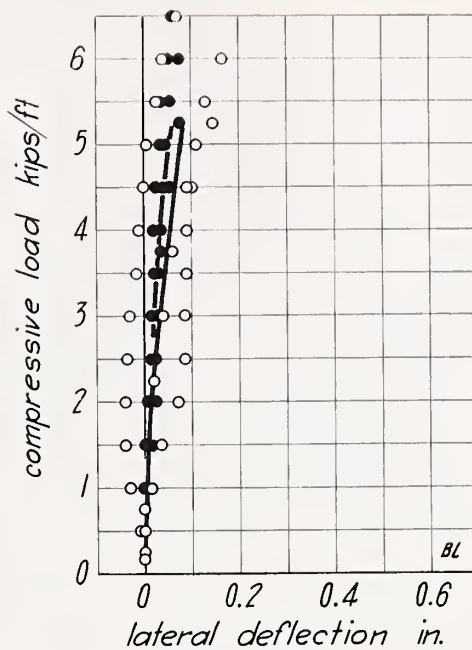
FIGURE 62.—Compressive load on wall BL.
