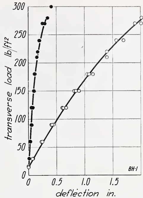
FIGURE 20.—Transverse load on wall BH-I, load applied to inside face.
