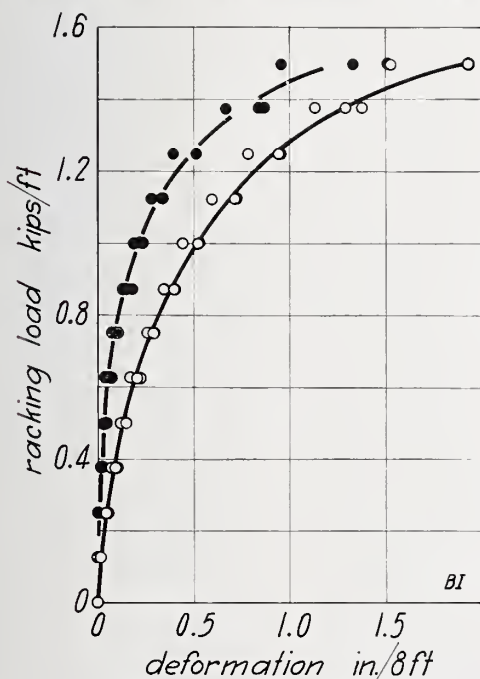
FIGURE 37.—Racking load on wall BI .
