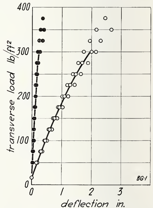
FIGURE 9. Transverse load on wall BG, load applied to inside face.
