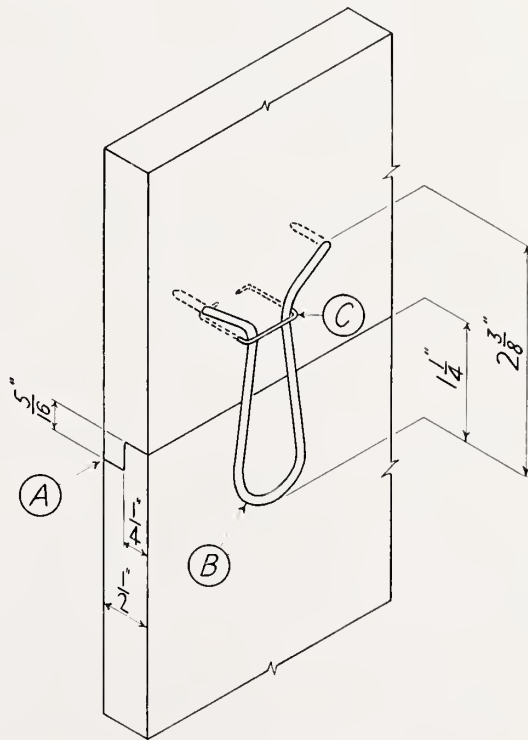
FIGURE 4.—"Lok-Joint" lath.
