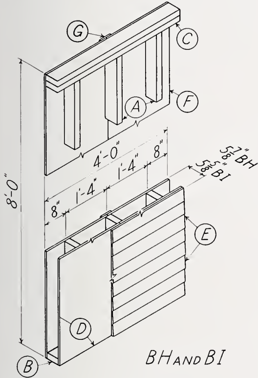
FIGURE 17.—Four-foot wall specimens BH and BI.
