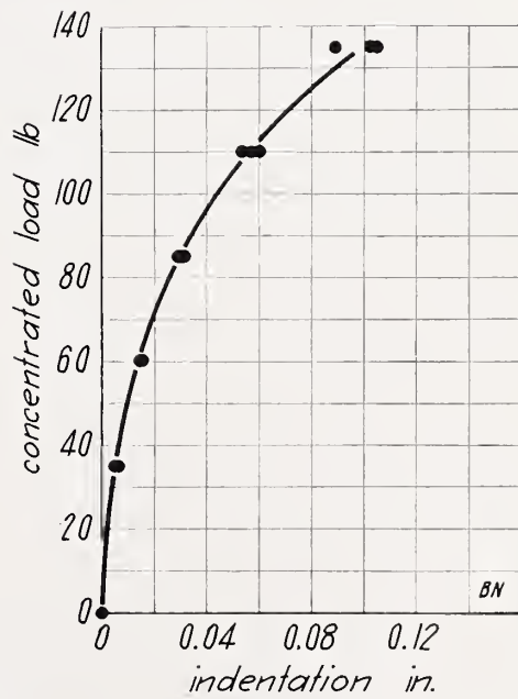
FIGURE 78.—Concentrated load on partition BN.
