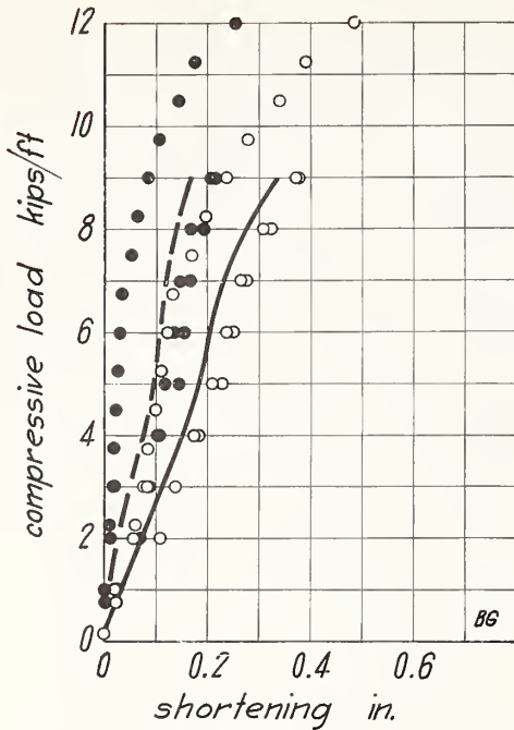
FIGURE 7.—Compressive load on wall BG.
