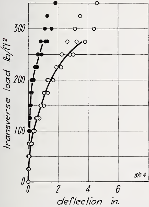
FIGURE 54.—Transverse load on wall BK, load applied to outside face.
