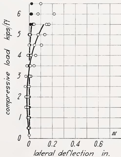
FIGURE 29.—Compressive load on wall BI .
