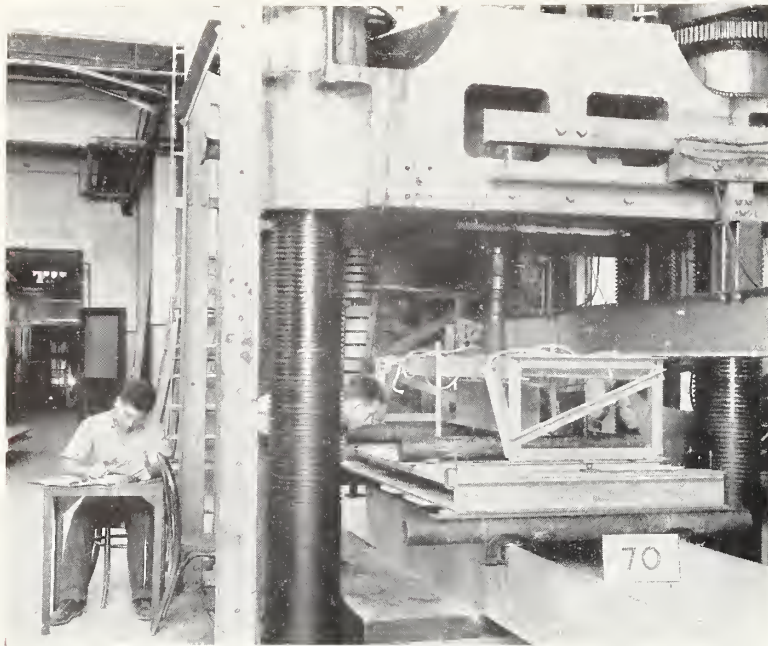
FIGURE 30.—Wall specimen BI-T6 under transverse load.
