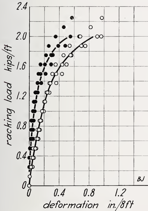
FIGURE 48.—Racking load on wall BJ .
