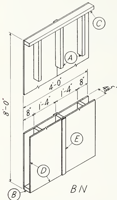
FIGURE 75.—Partition specimen BN .
