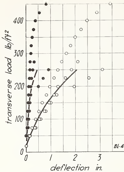
FIGURE 64.—Transverse load on wall BL, load applied to outside face.
