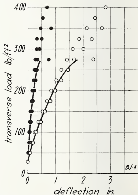
FIGURE 43.—Transverse load on wall BJ, load applied to outside face.
