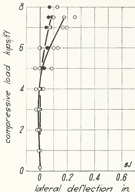
FIGURE 41.—Compressive load on wall BJ.
