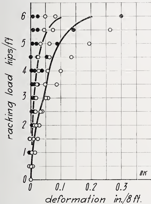
FIGURE 59.—Racking load on wall BK .
