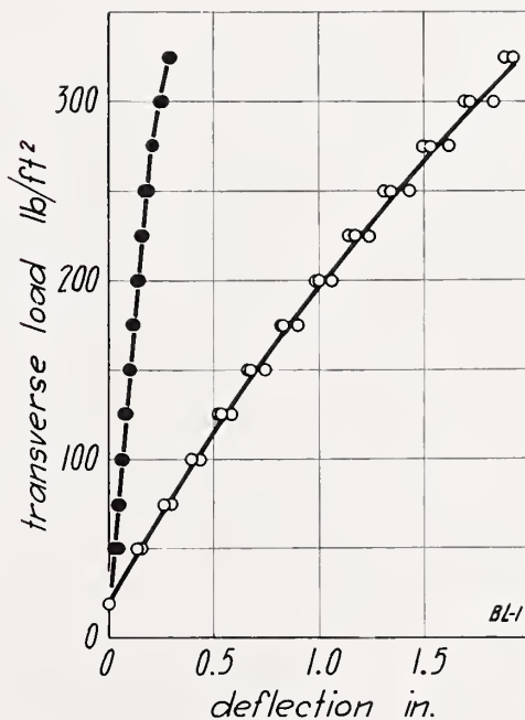
FIGURE 63.—Transverse load on wall BL, load applied to inside face.
