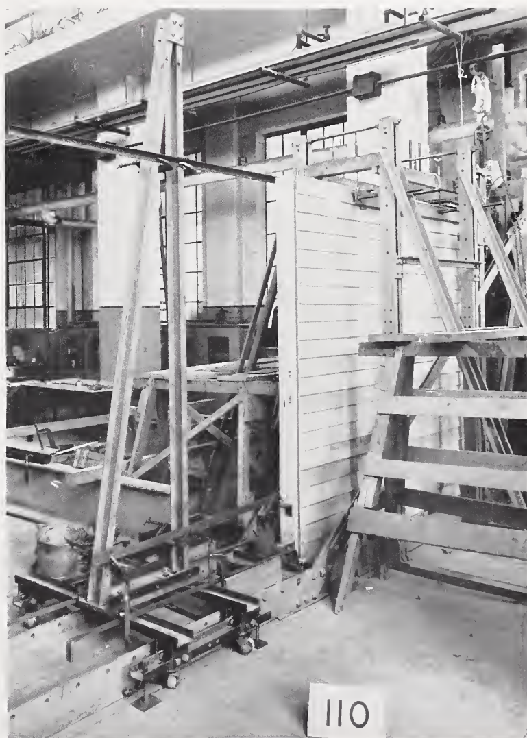
FIGURE 15.—Wall specimen BG-R1 , under racking load.
