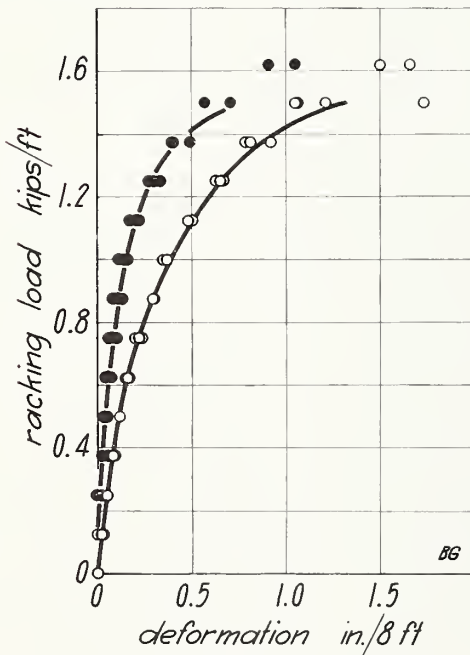
FIGURE 16.—Racking load on wall BG .
