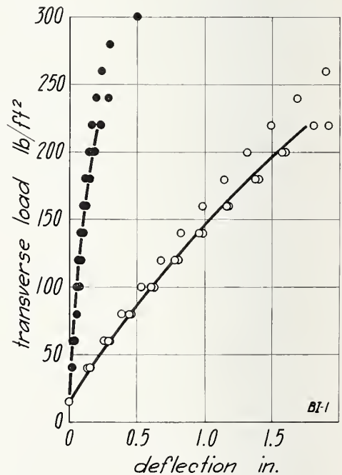
FIGURE 31.—Transverse load on wall BI , load applied to inside face.
