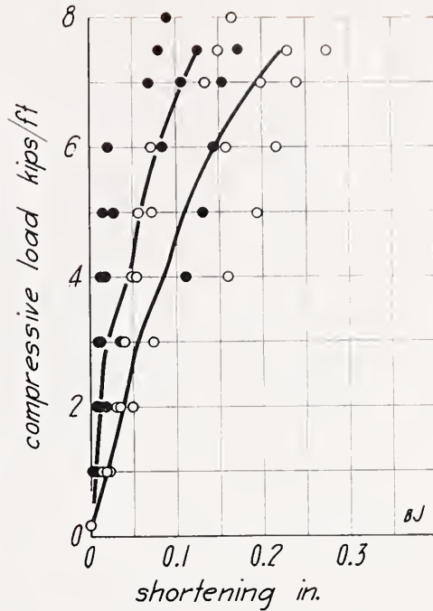
FIGURE 40.—Compressive load on wall BJ .
