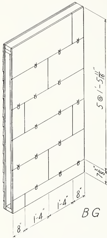
FIGURE 6.—Four-foot wall specimen BG.
