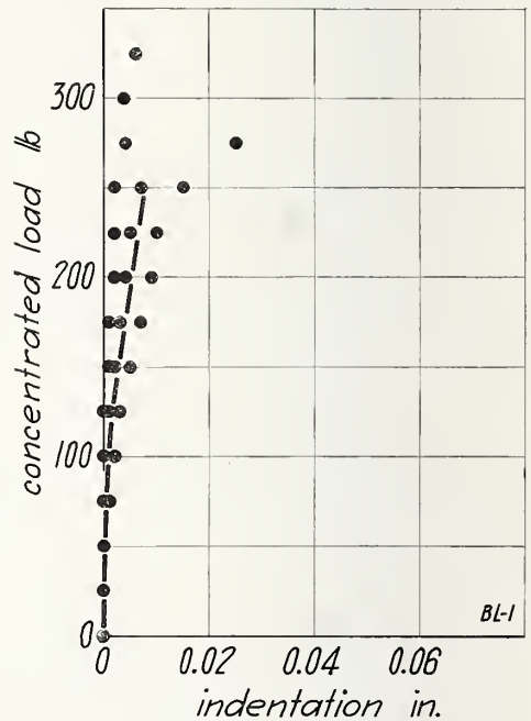
FIGURE 65.—Concentrated load on wall BL, load applied to inside face.
