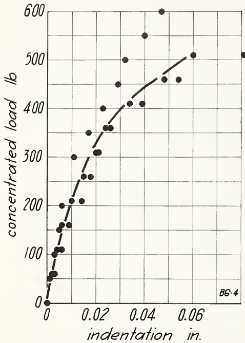
FIGURE 12.—Concentrated load on wall BG , load applied to outside face.
