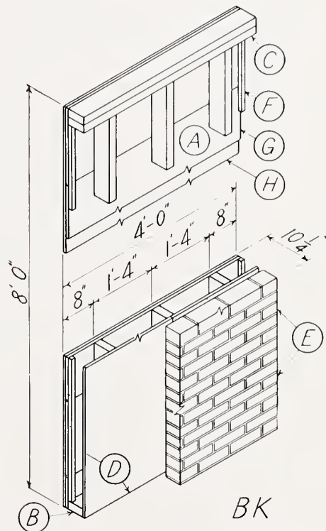
FIGURE 49.—Four-foot wall specimen BK .
