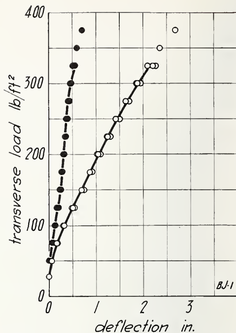
FIGURE 42.—Transverse load on wall BJ, load applied to inside face.
