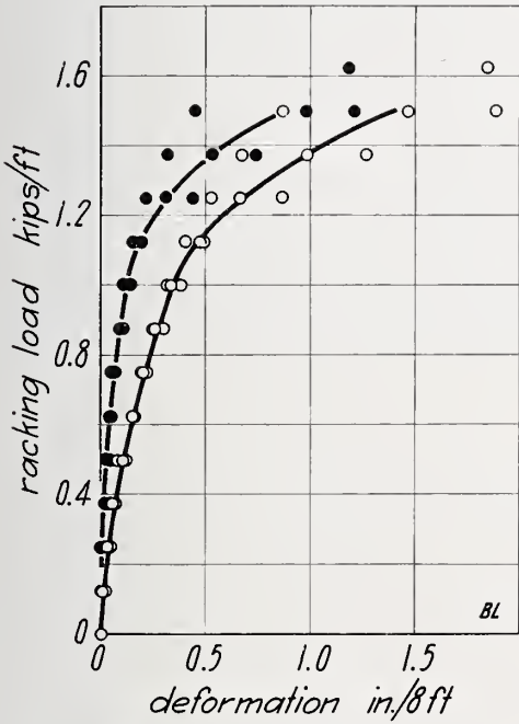
FIGURE 70.—Racking load on wall BL .
