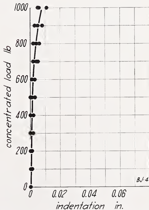
FIGURE 45.—Concentrated load on wall BJ, load applied to outside face.
