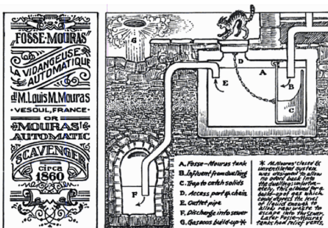
Fig 1. Schematic of an early-design septic tank from 1860. (from http://djwl.co.uk/blog/brief-history-septic-tanks/ )
