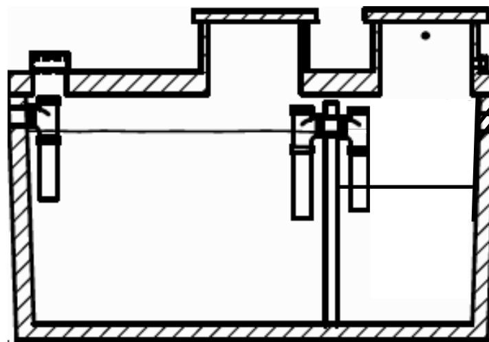
Septic and Dosing Two Compartment Combo Tank
