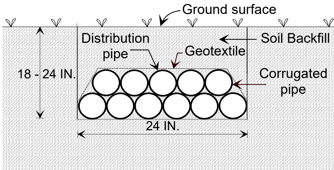
Figure 1b. Typical Multiple-pipe Gravelless Drainfield, Cross-Section
