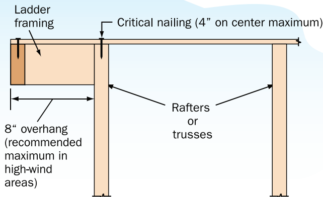
Ladder framing at gable ends.
