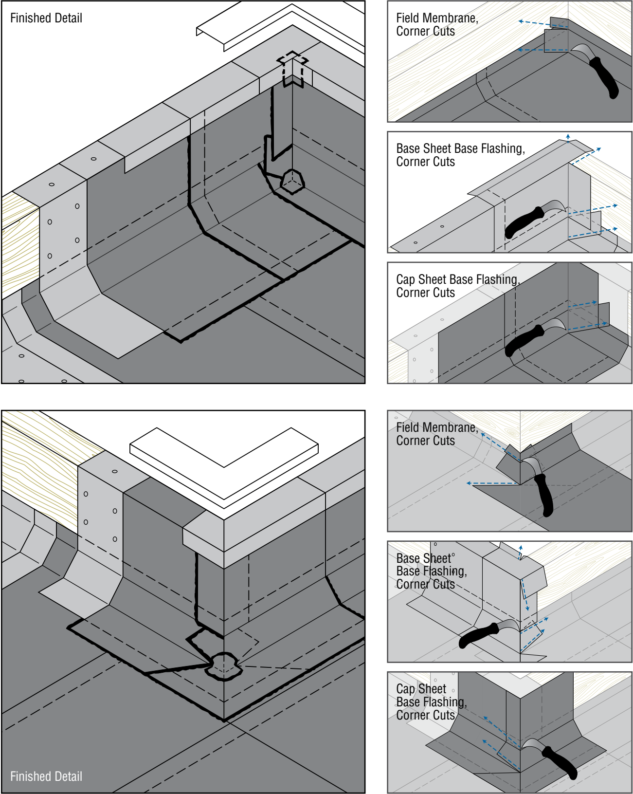
CT-10 Base Flashing on Parapet Wall, Outside Corner
