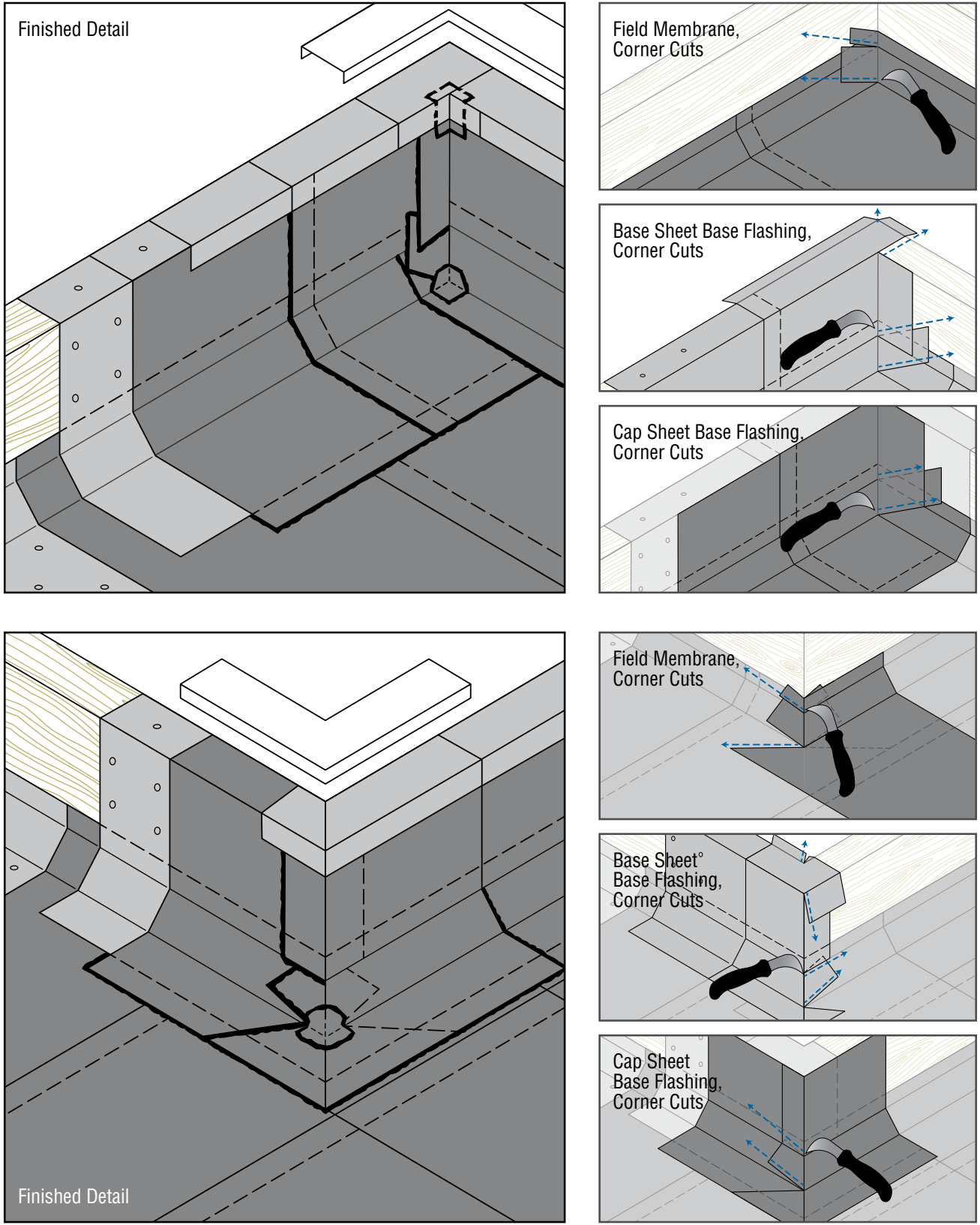
CT-10 Base Flashing on Parapet Wall, Outside Corner
