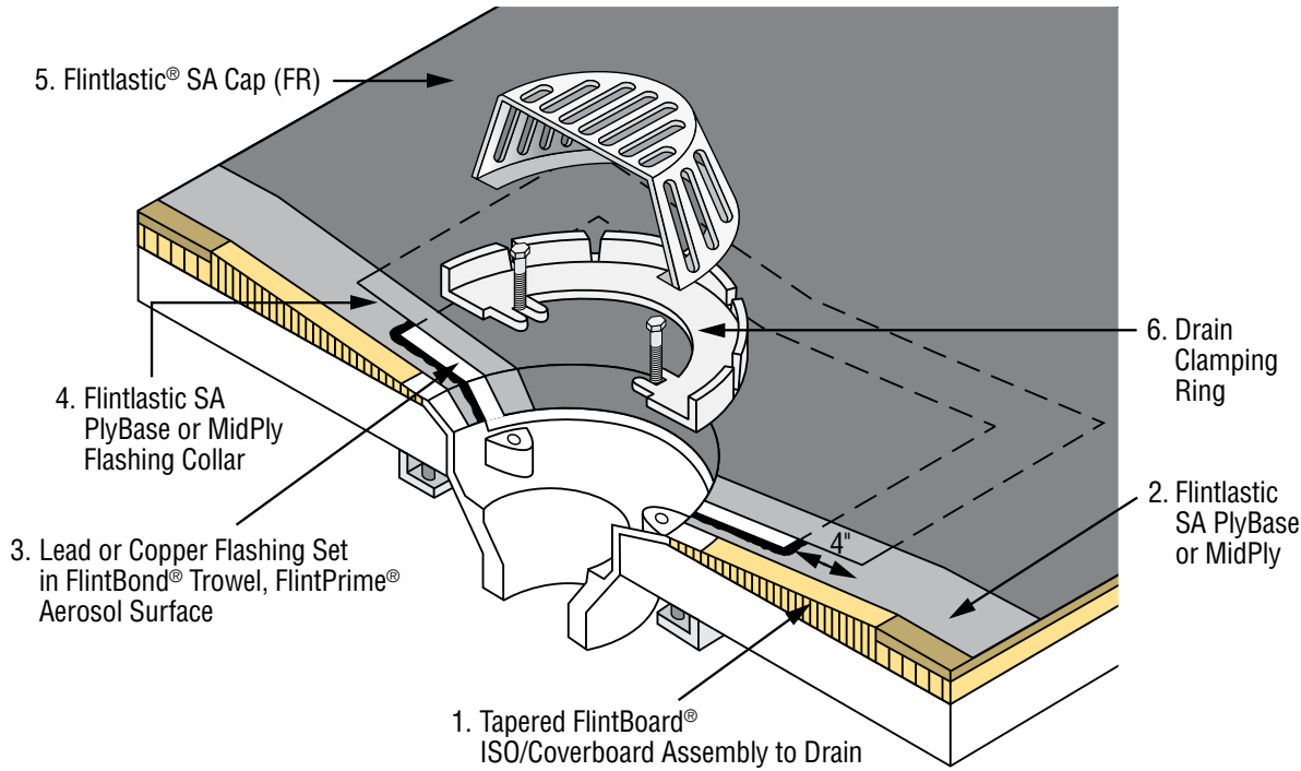
CT-12 Drain Flashing
