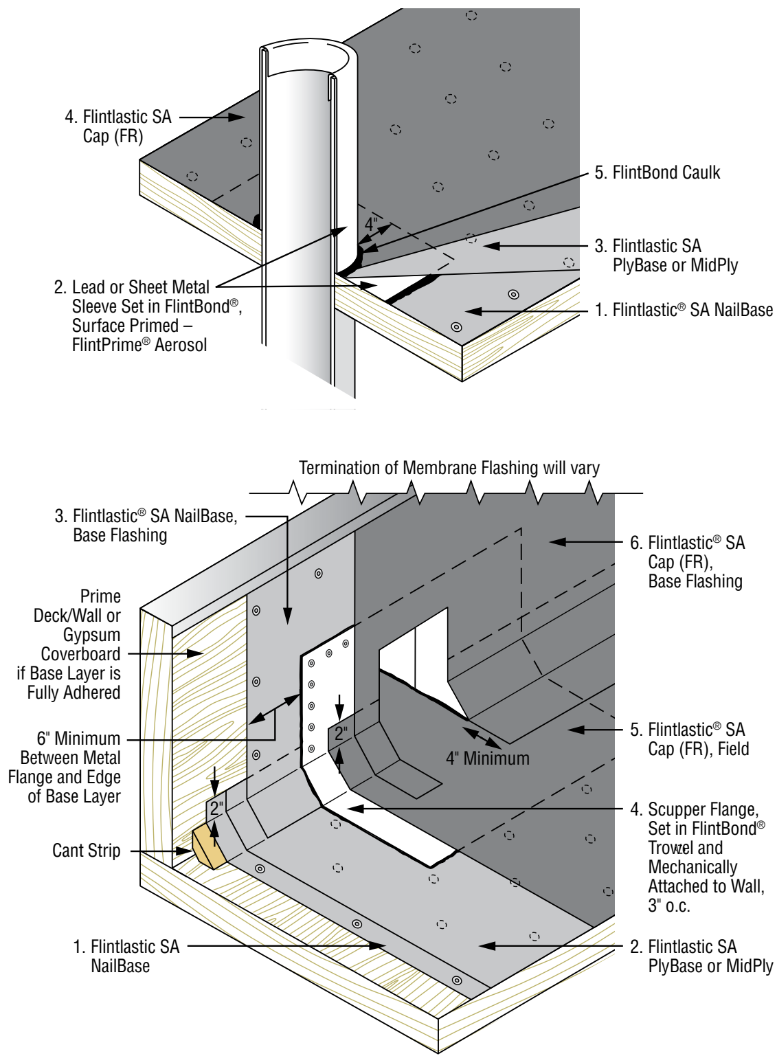
CT-11 Through-Wall Scupper Flashing
