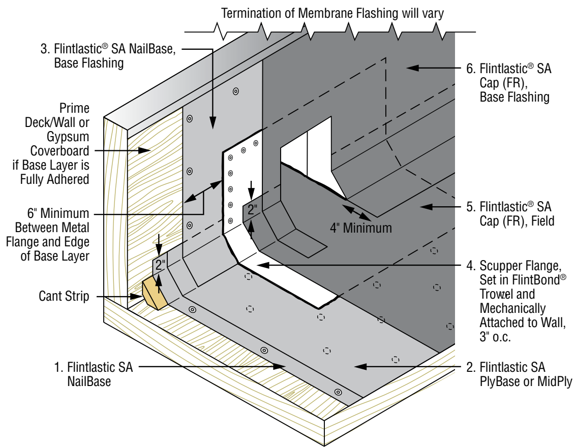
CT-11 Through-Wall Scupper Flashing
