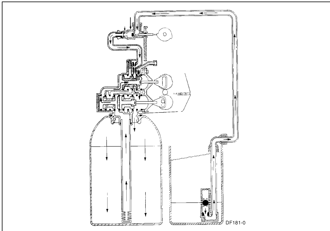
Figure 41: Brine Draw
