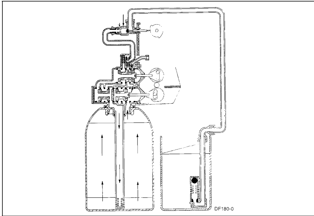
Figure 40: Backwash Position
