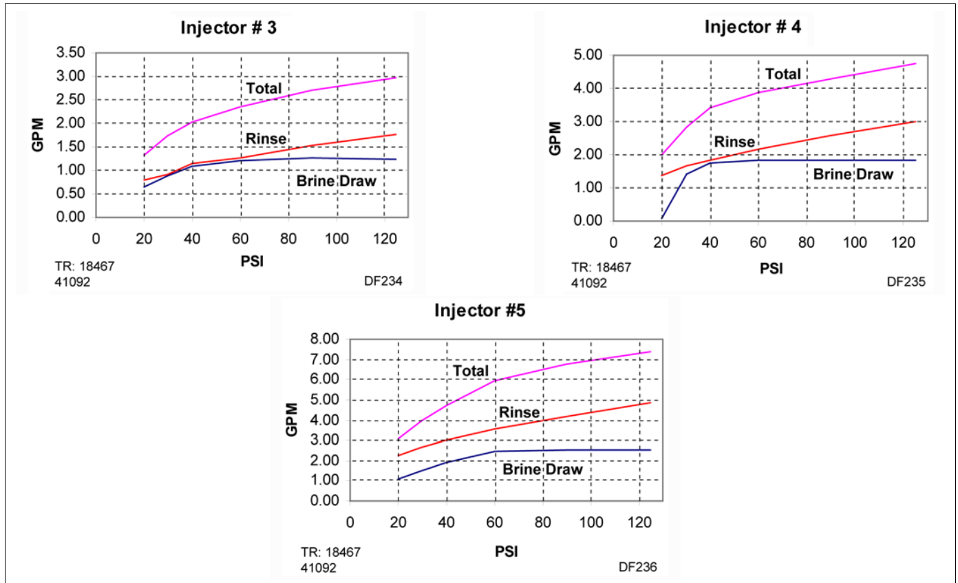
Figure 57: 9500–1700 Series Injectors
