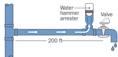
Fig 1: Shut-off valve at END of long pipe run
