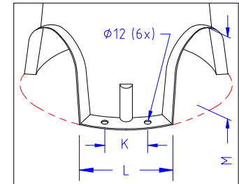
DETAIL BASE
