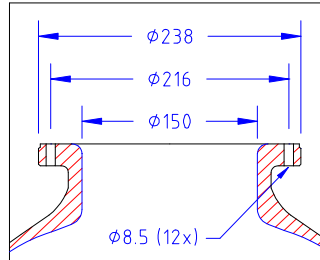
DETAIL 6" FLANGE
