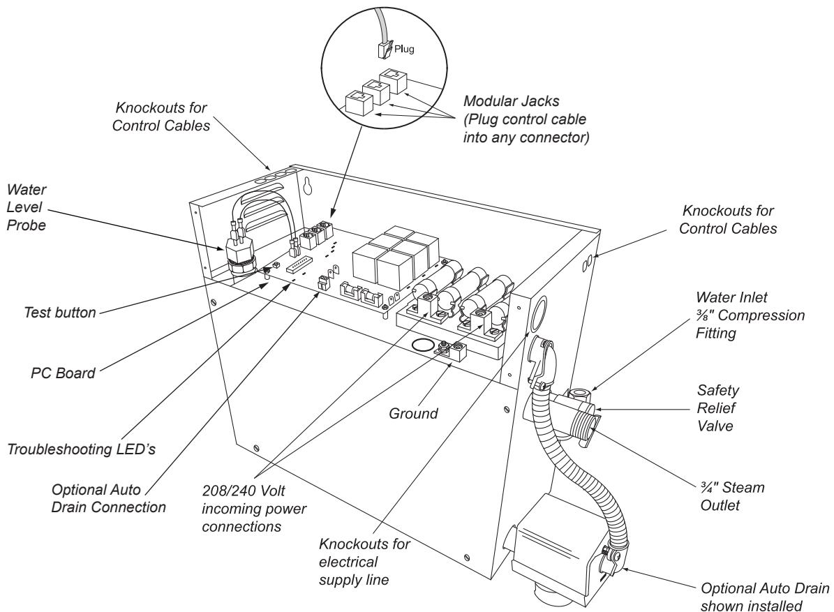
Figure 2 - Internal Electrical Connections
