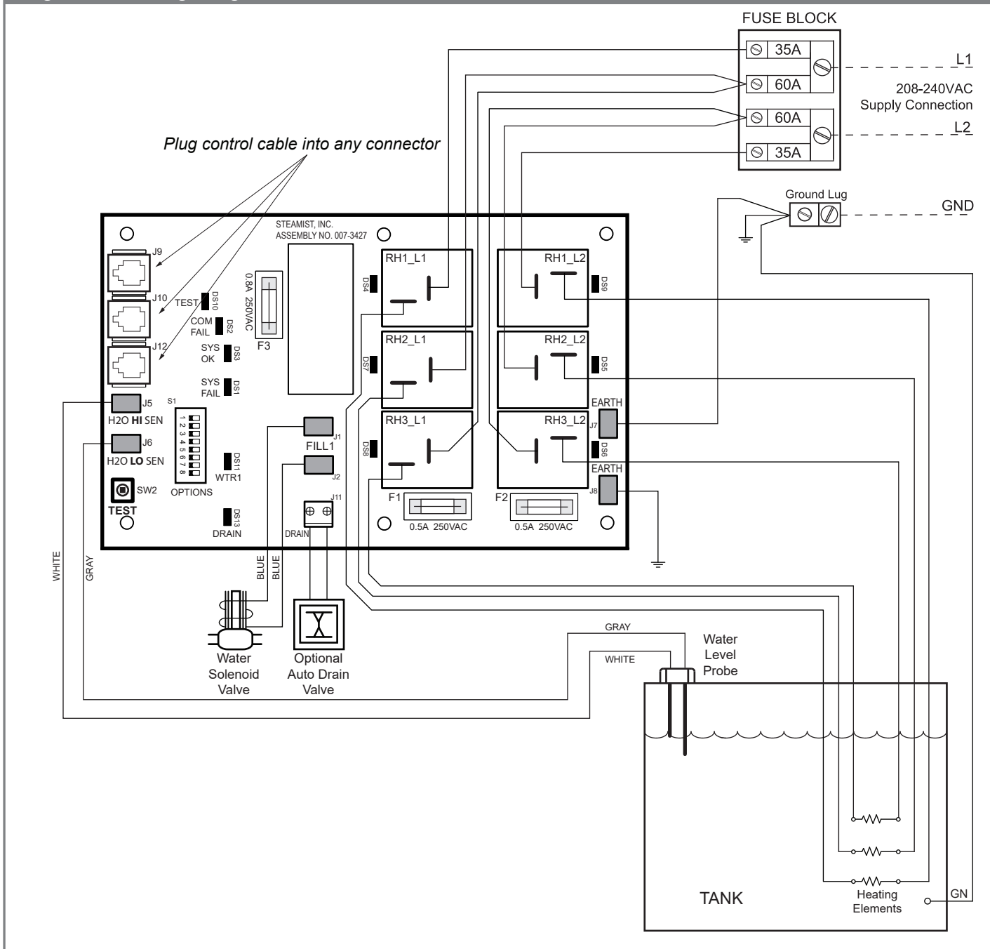
Figure 5 - Wiring Diagram
