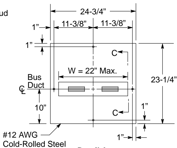
Detail A End Flange Plate (customer supplied)
