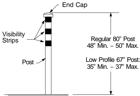
Figure 24 Steel Barrier Post (see Table 4)
