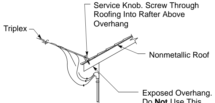
Figure 4-28 Cable (Using Triplex) Exposed Overhang. Do Not Use This Construction Where Overhang Is Boxed In
