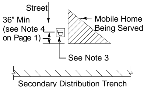
Figure 2 Pedestal (preferred location)
