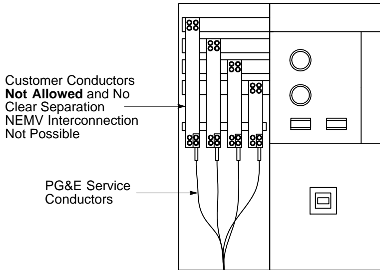
Figure 7 Pull Section with No Clear Separation
