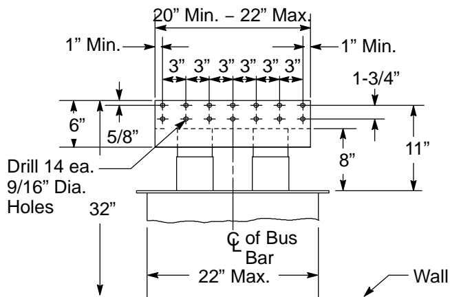
Section F-F Tie Bar Connection 1/4" x 6" x 20" Long Copper (two per phase and one per neutral required) (customer supplied)
