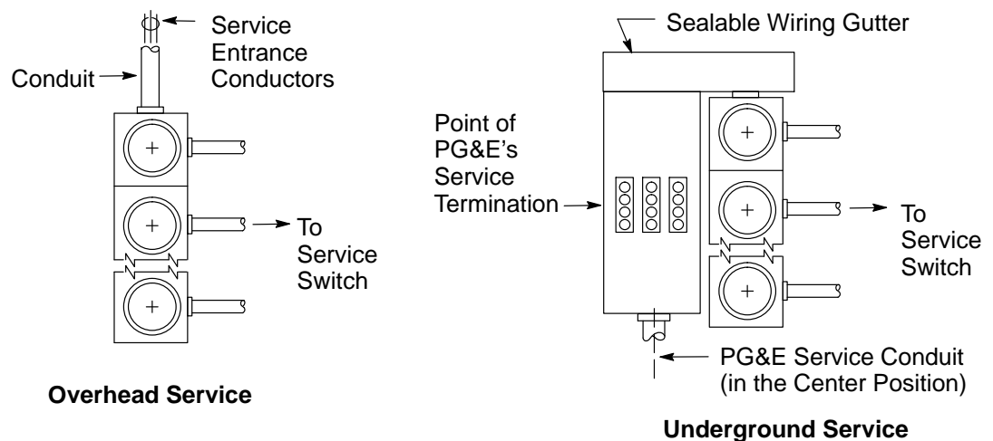
Overhead Service Underground Service Vertical Meter Trough Installation: Five Meters or Less
