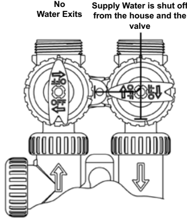
Figure 4 SHUT OFF MODE
