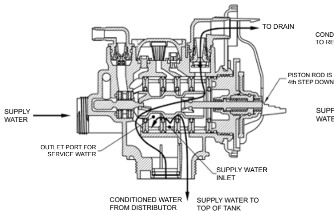
flow diagram...rinse
