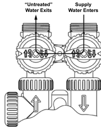
Figure 2 BYPASS OPERATION
