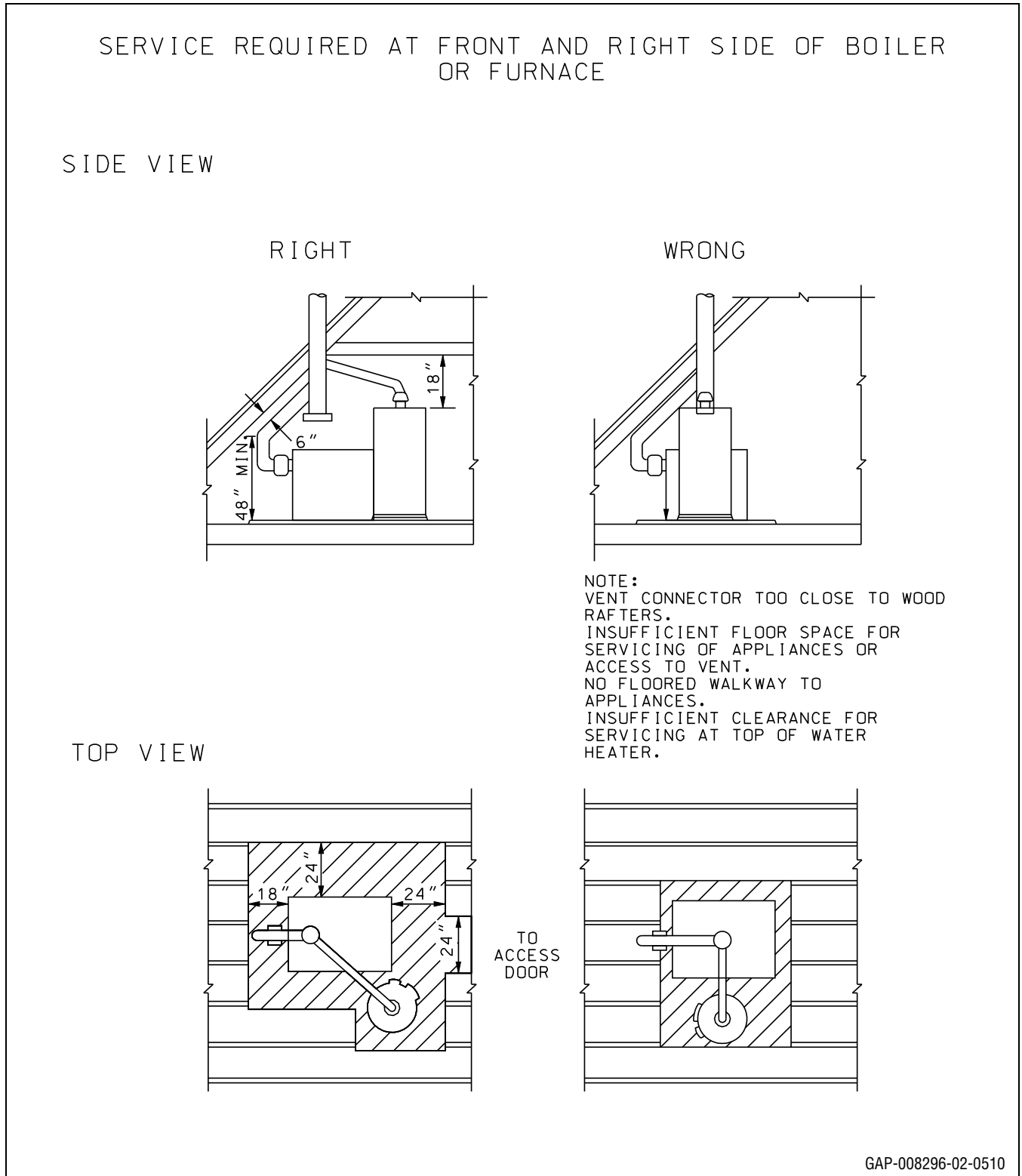
Figure 4.5: Examples of Minimum Attic Clearances
