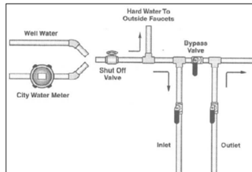
Diagram 6: Three-Way Bypass Plumbing
