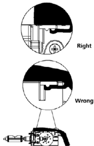
Diagram 13: Controller Tab Lock Detail
