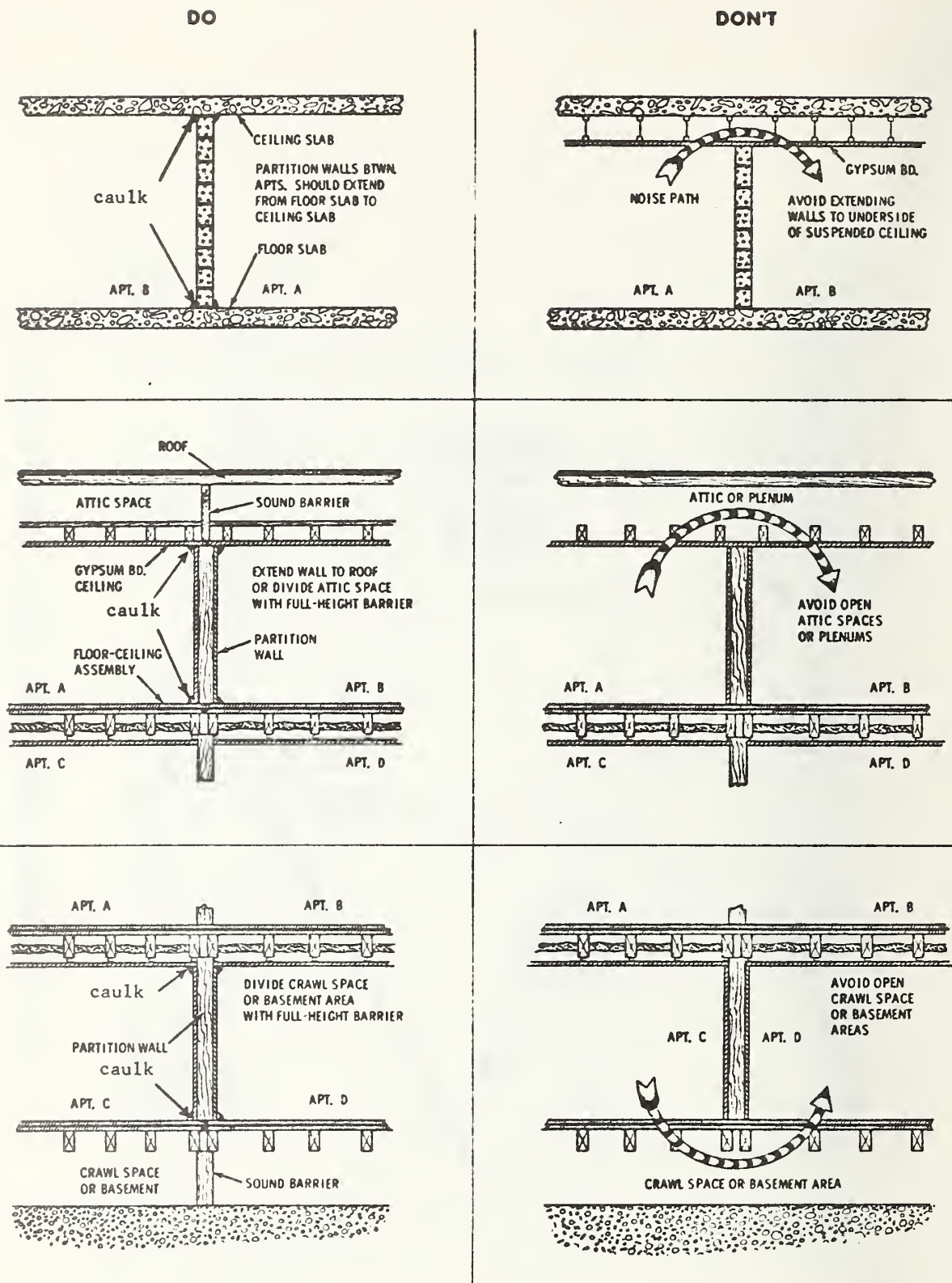
FIG. 4-14 METHODS OF CONTROLLING FLANKING SOUND TRANSMISSION PATHS.
