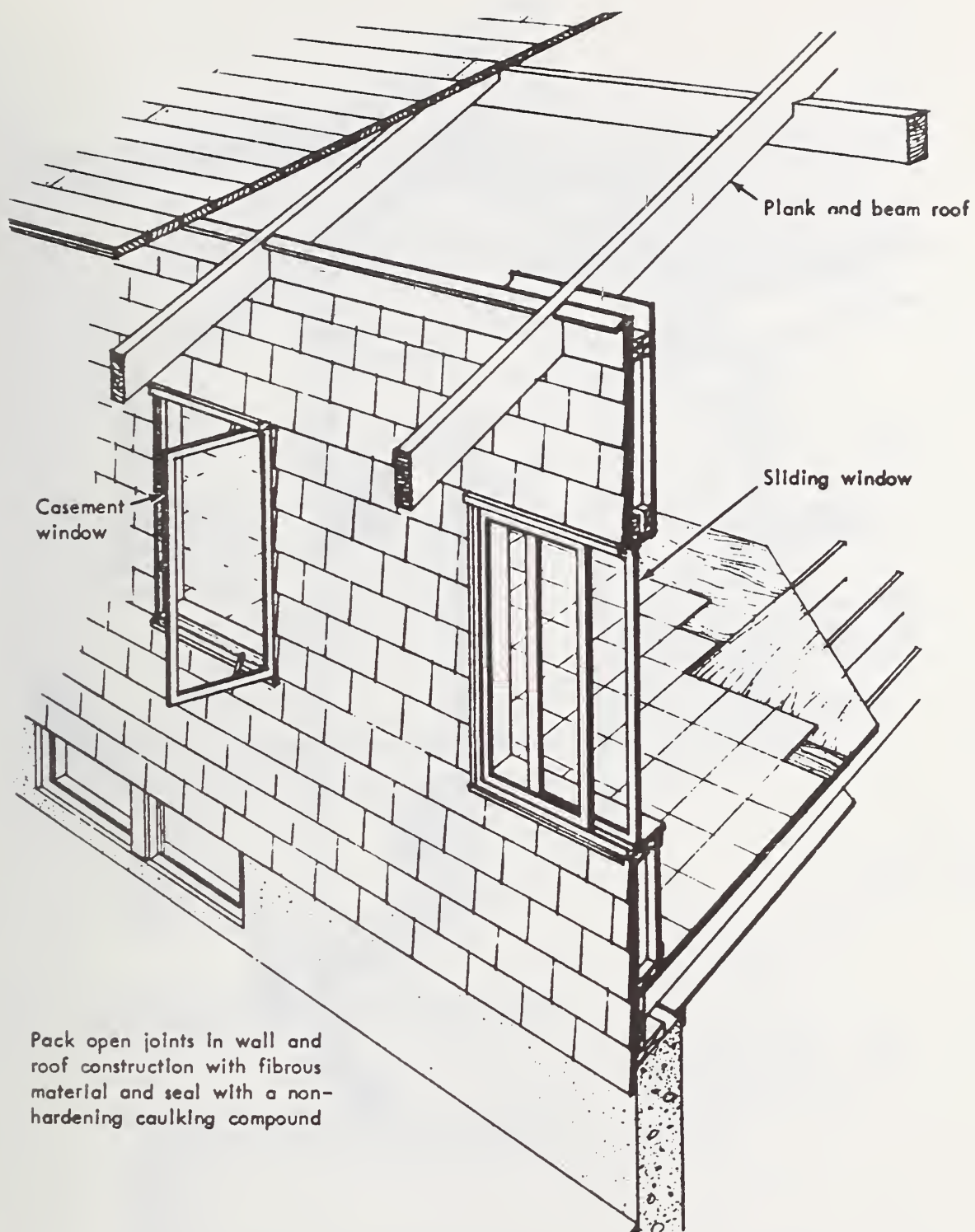
FIG 5-3 HOUSE WITH BASEMENT AND PLANK AND BEAM ROOF.
