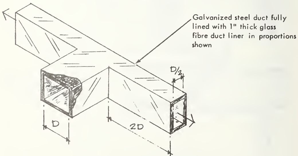
FIG. 5-6 CRAWL SPACE MODIFICATIONS.
