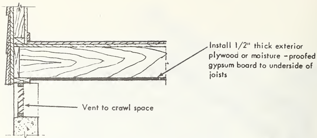
a - Added floor construction
