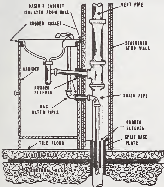
FIG. 4-25 PROPER INSTALLATION OF BATH TUBS AND WASH BASINS.
