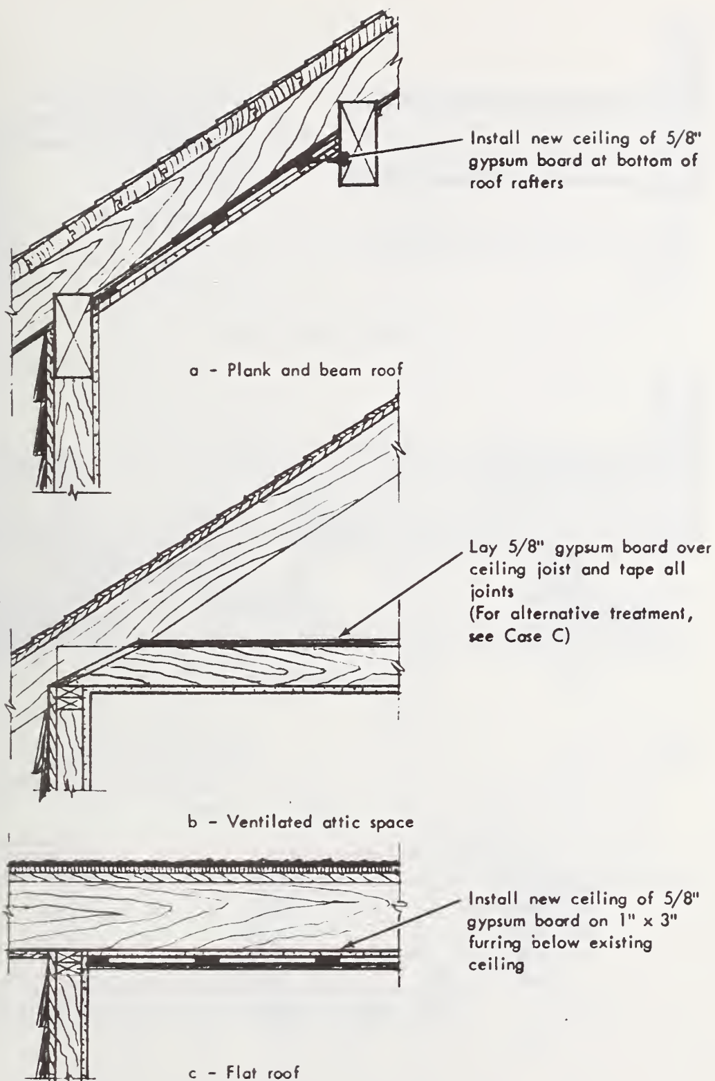
FIG. 5-5 ROOF AND CEILING MODIFICATIONS.
