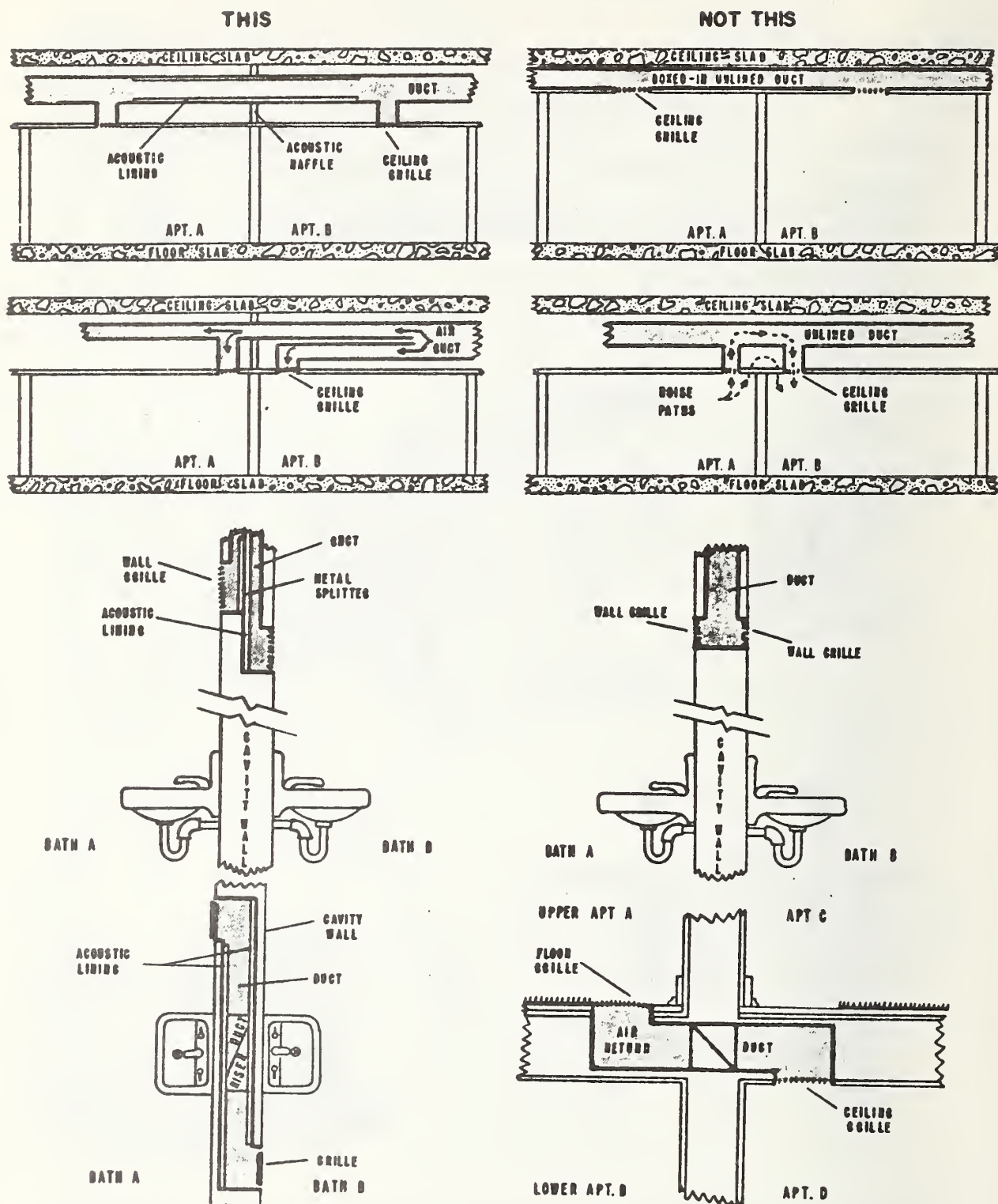
FIG. 4-22 METHODS OF CONTROLLING CROSS TALK AND THE TRANSMISSION OF FLANKING NOISE IN DUCTS.
