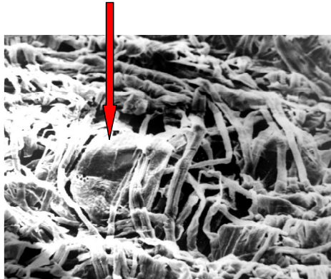
Vessel element in a sanitary tissue paper sheet
