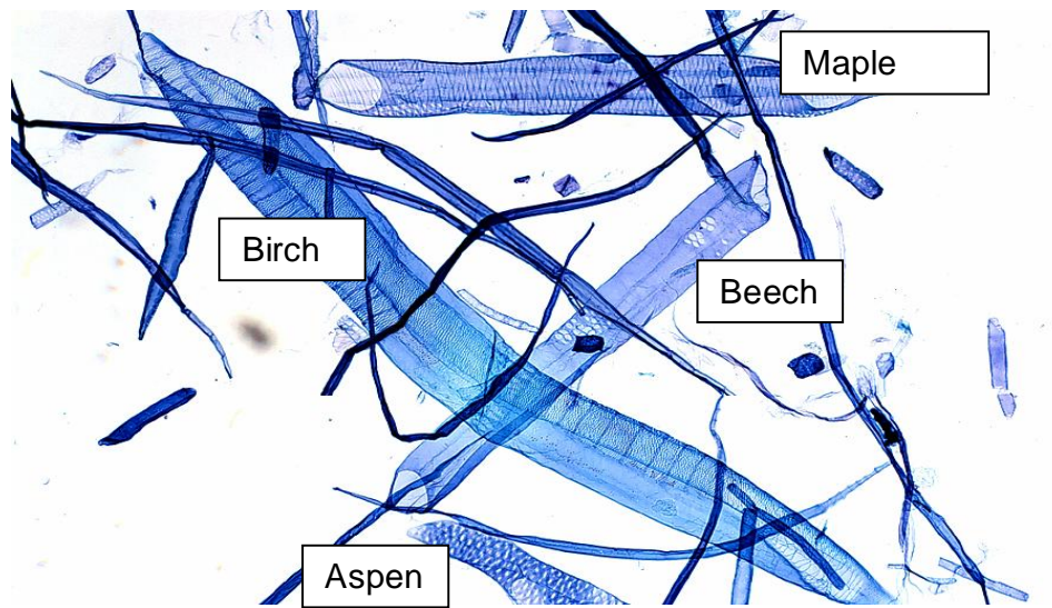
Vessels of different hardwood pulps (Source: PAPRICAN, undated)
