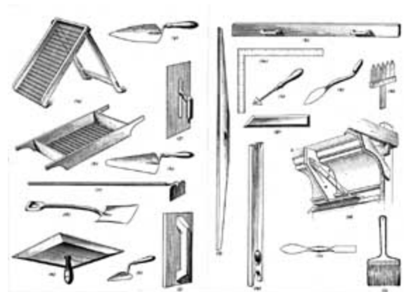
Many of these traditional plastering tools are still used today. Drawing: NPS files.
