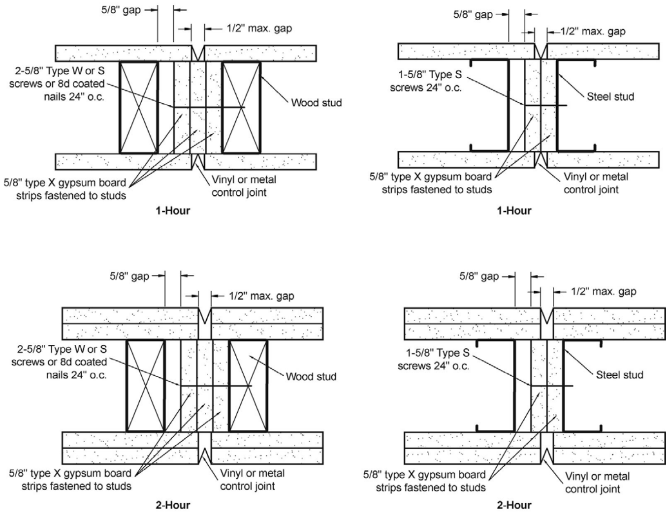
FIGURE 1—CONTROL JOINT DETAILS
