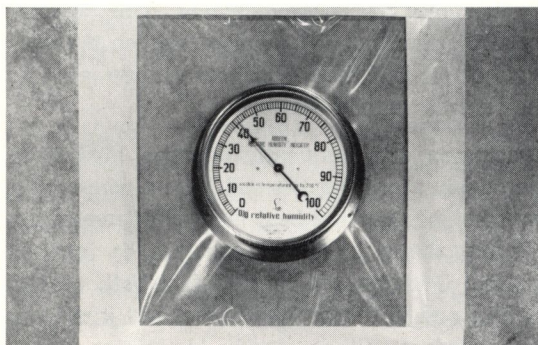
A relative humidity meter, placed under polyethylene sheeting, sealed at the edges with tape or adhesive, should be used on new above-grade concrete before installing materials affected by moisture. After a suitable period, a reading of 80% RH or lower indicates satisfactory dryness.
