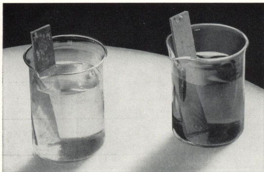
Immersion for 2 hours in a 2 per cent solution of sodium hydroxide determines the color permanency of pigments in tiles specified for use over, on-, and below-grade concrete. The beaker at the right shows bleeding of colors from pigments that are not alkali resistant.
