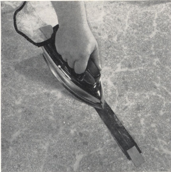
An electric iron and aluminum foil in experienced hands can weld seams in vinyl sheet flooring and, by eliminating dirt traps, create a "cleaner," more cleanable floor.
