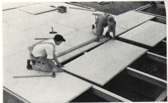
Among the advantages of 2-4-1 T & G Plywood are: fewer individual pieces to handle, register holes can be cut without framing, fewer joints for air drafts, less labor and material costs, uncluttered basement ceilings, and no underlayment needed beneath resilient flooring.
