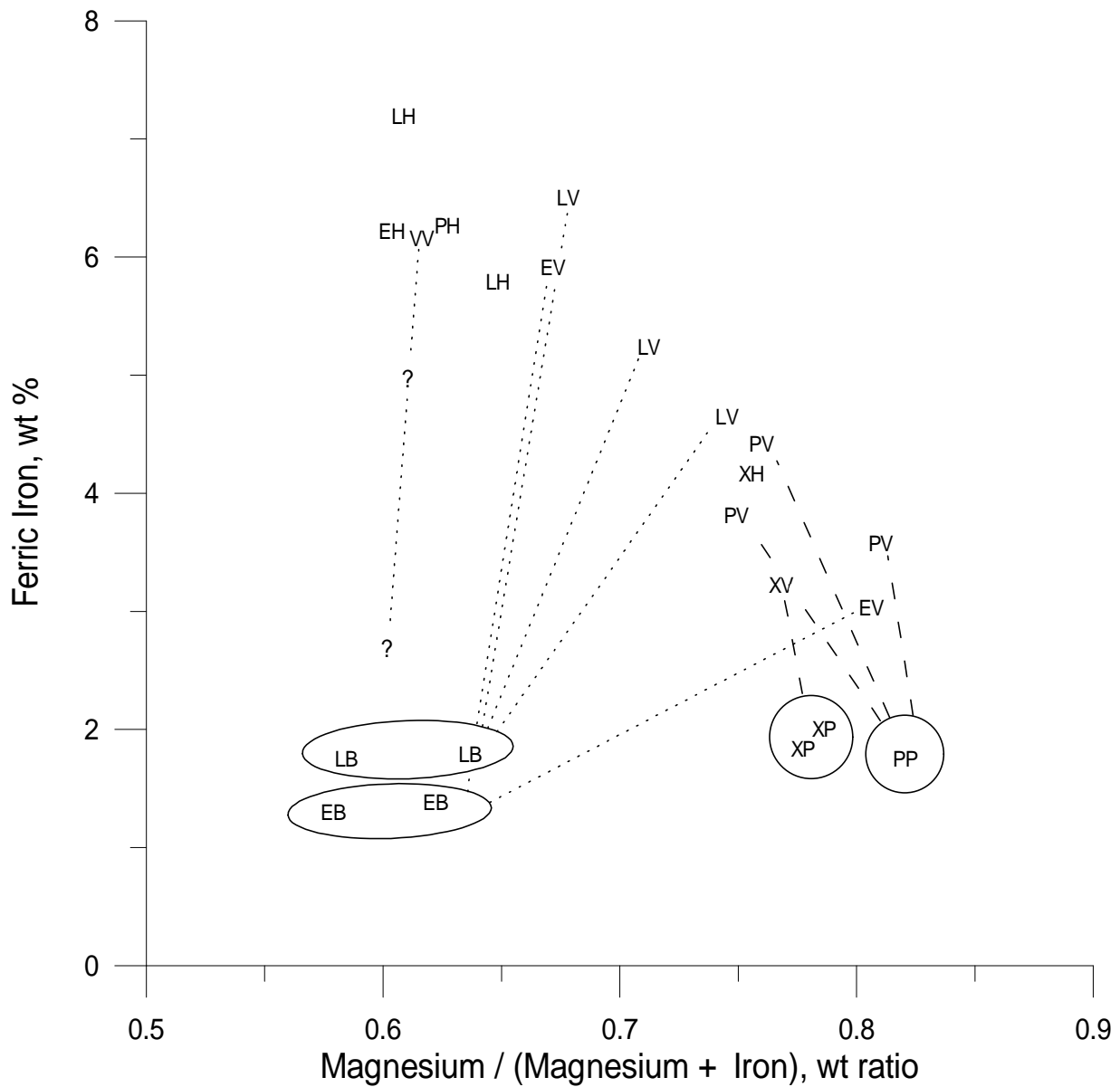
Figure 3. Distribution of magnesium, total iron, and ferric iron in vermiculite, mixed-layer mica vermiculite (hydrobiotite and hydrophlogopite), and mica (biotite and phlogopite). Parent micas are circled; tielines match parent micas with vermiculite from the same localities. Mixed-layer symbols do not have tielines. Data from Table 4.
