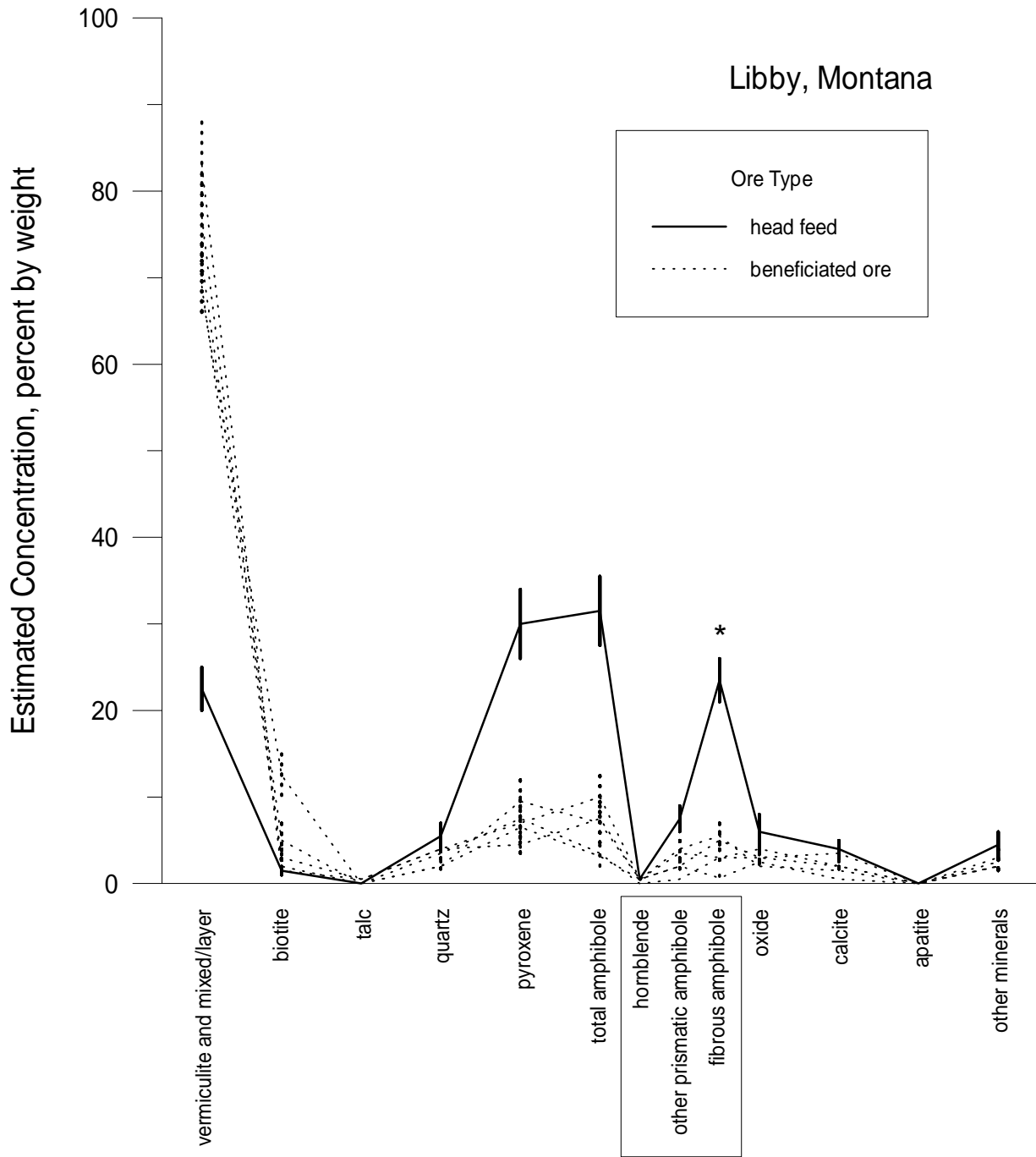
Figure 2A. Mineral composition of vermiculite ore (data from Atkinson and others, 1982). Data include head feed (solid line), and five grades of beneficiated ore (dotted lines) from the W.R. Grace mine at Libby, Montana. The graph shows three types of amphiboles (outlined) that make up total amphiboles. Asterisk indicates fibrous amphiboles.
