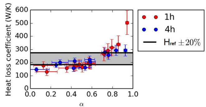
Fig. 11. H_{\text{QUB}} = f(\alpha) in the Energy House at the University of Salford. The red and blue dots are obtained respectively for durations of 1 h and 4 h. The solid black lines delimiting the grey zone corresponds to \pm 20\% of the reference value. (For interpretation of the references to color in this figure legend, the reader is referred to the web version of this article.)
