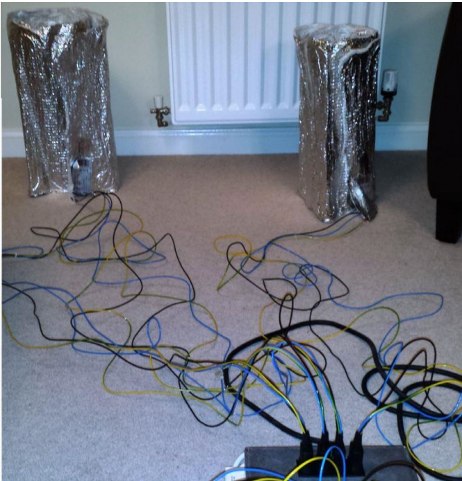
Fig. 1. 110 W aluminum heat mats connected to boxes allowing to switch simultaneously on or off at requested times.
