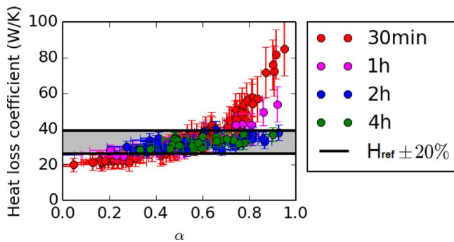
Fig. 10. H_{\text{QUB}} = f(\alpha) in SGR bungalows. The red, magenta, blue and green dots are obtained respectively for durations of 30 min, 1 h, 2 h and 4 h. The solid black lines delimiting the grey zone corresponds to \pm 20\% of the reference value. (For interpretation of the references to color in this figure legend, the reader is referred to the web version of this article.)
