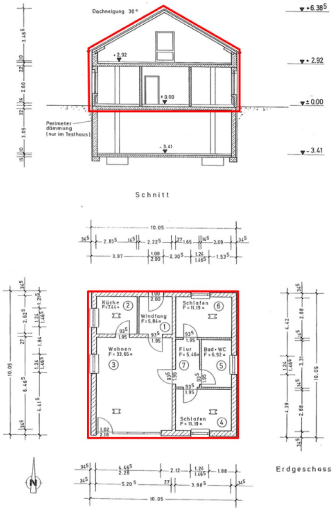
Fig. 13. Section and ground floor plan of the test house.
