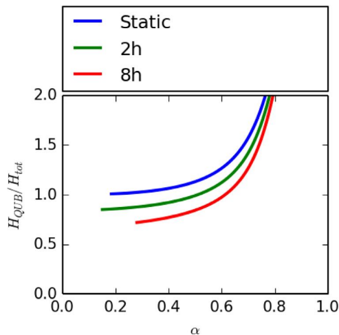
Fig. 9. H_{QUB}/H_{tot} = f(\alpha) for a heating and cooling durations of 4 h in the EWI case, calculated using a numerical resolution of the quadrupole model. The blue line is the result starting from a static initial state, the green for 2 h of cooling before the QUB and the red corresponds to 8 h of cooling. (For interpretation of the references to color in this figure legend, the reader is referred to the web version of this article.)
