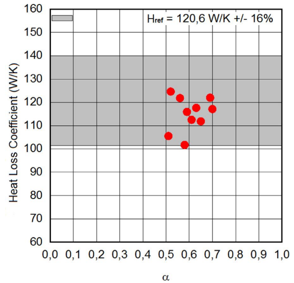
Fig. 14. Measured heat loss coefficients in dependence of the \alpha -value.
