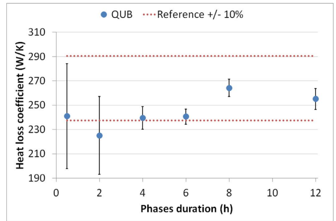
Fig. 5. Results of QUB tests of different durations at the Energy House in Salford. The blue dots are the HLC results obtained via the QUB method as a function of the heating and cooling durations and the dashed red lines delimit the reference value \pm 10\% . (For interpretation of the references to color in this figure legend, the reader is referred to the web version of this article.)
