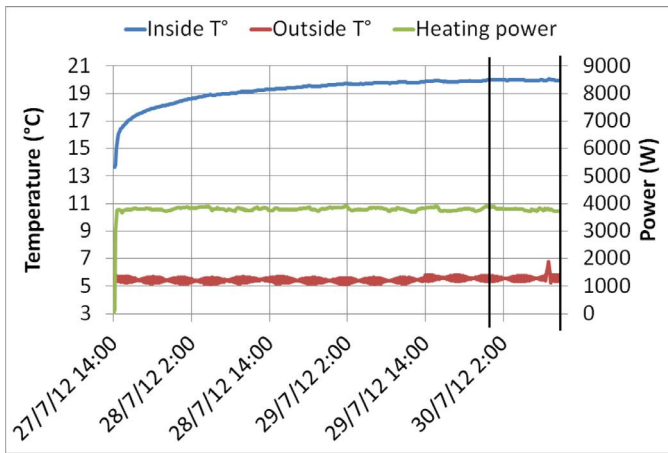
Fig. 3. Steady-state measurements at the Energy House. The blue line is the average inside temperature, the red is the outside temperature and the green is the heating power. The period used for average is delimited by the two solid black lines. (For interpretation of the references to color in this figure legend, the reader is referred to the web version of this article.)
