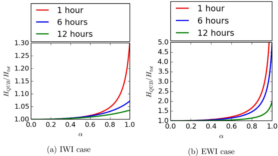
Fig. 8. H_{QUB}/H_{tot} = f(\alpha) for IWI wall (a) and EWI wall (b), calculated using a numerical resolution of the quadrupole model. The blue lines are the results for 6 h of heating and cooling, the green ones for 12 h and the red for 1 h. (For interpretation of the references to color in this figure legend, the reader is referred to the web version of this article.)
