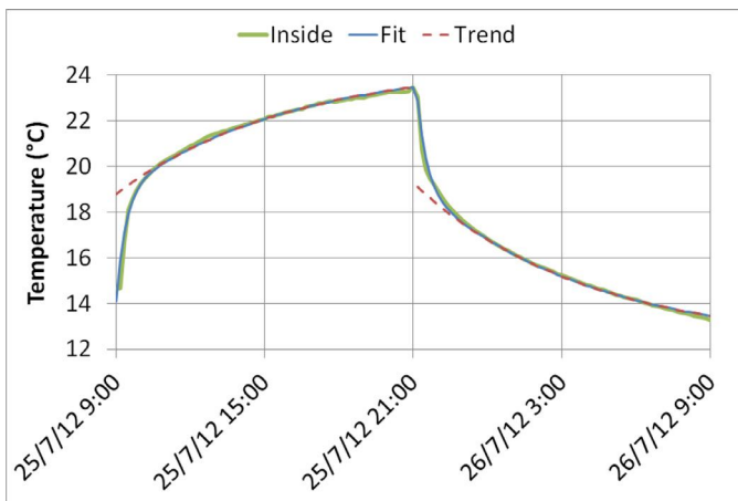
Fig. 4. QUB test at the Energy House. The solid green lines represents the average inside temperature, the solid blue is the best fit obtained using a two time constant model and the dashed red is the trend using only the largest time constant of the best fit. (For interpretation of the references to color in this figure legend, the reader is referred to the web version of this article.)
