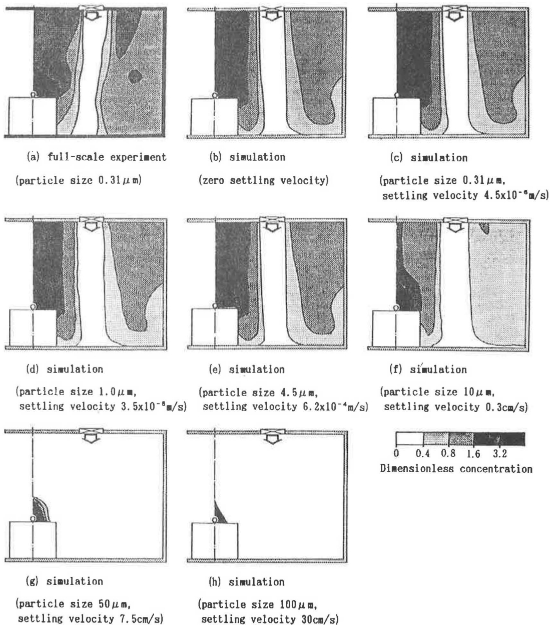
Figure 10 Comparisons of contaminant distributions of Type 2 room model (with obstacle, gravitational settling velocity is considered).
