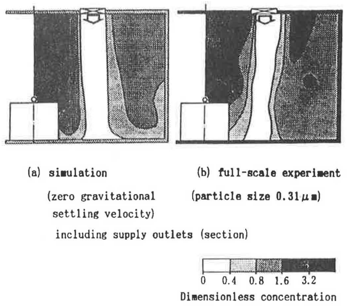
Figure 8 Comparison of contaminant distributions of Type 2 room model (with obstacle).
