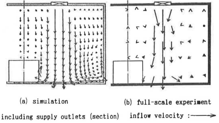
Figure 7 Comparison of flow fields of Type 2 room model (with obstacle).
