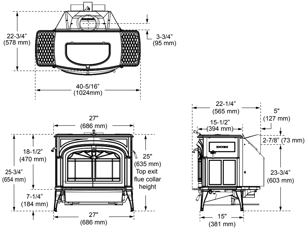
Figure 1 - Encore® 2040 dimensions.
