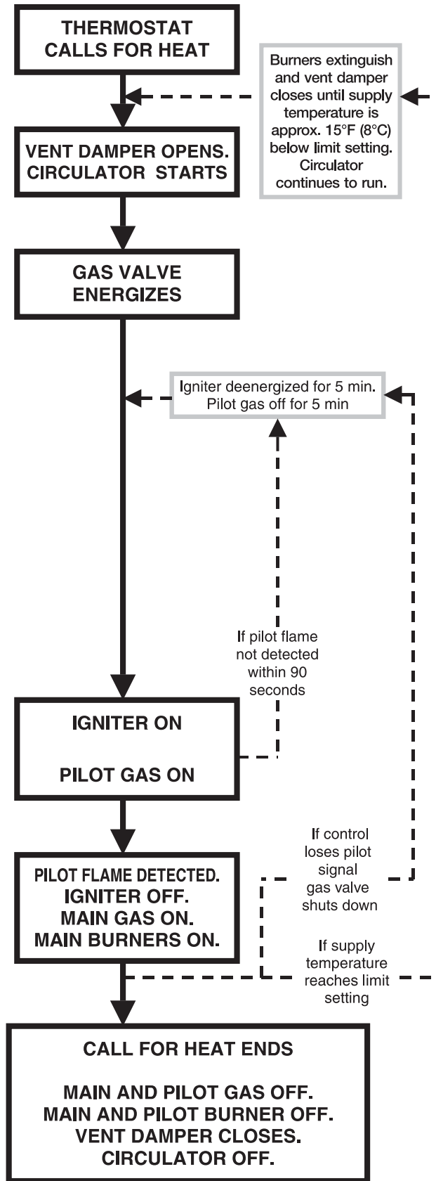
Figure 4: Intermittent Ignition Sequence of Operation
