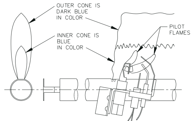
Figure 5: Intermittent Ignition Pilot Configuration and Flames
