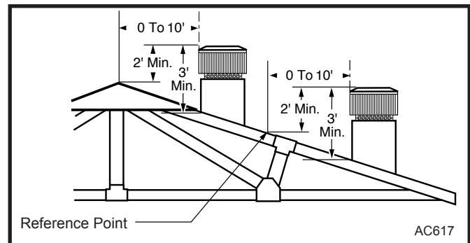
Fig. 2 The 2'-3'-10' rule for chimneys.
