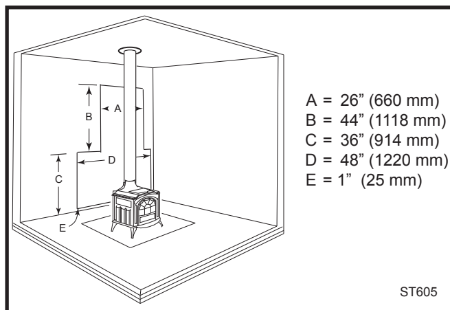
Fig. 19 A top-exit stove with a wall shield only no pipe or stove heat shields). A 26" wide section of rear wall shield must be centered behind the connector.
