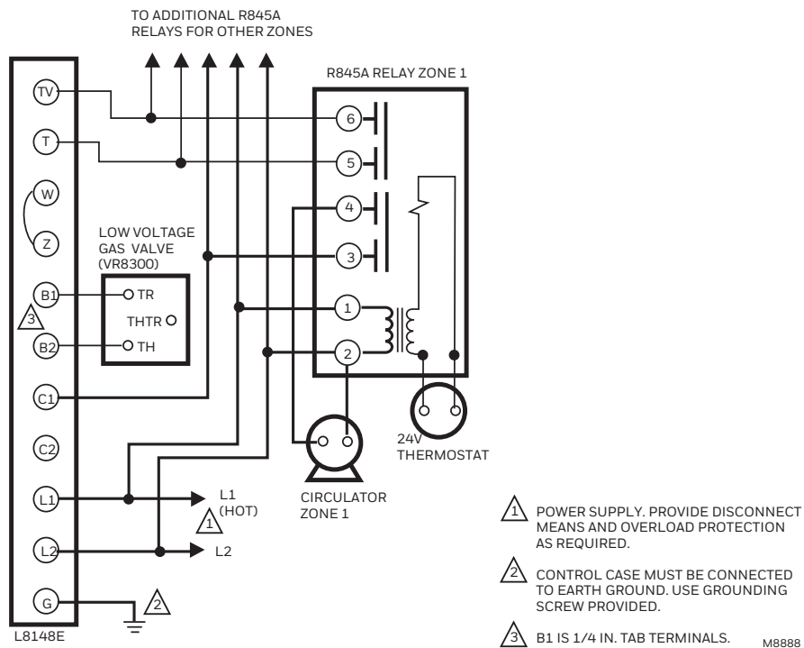
Fig. 10. Wiring L8148E in multizone system with R845 switched circulator.
