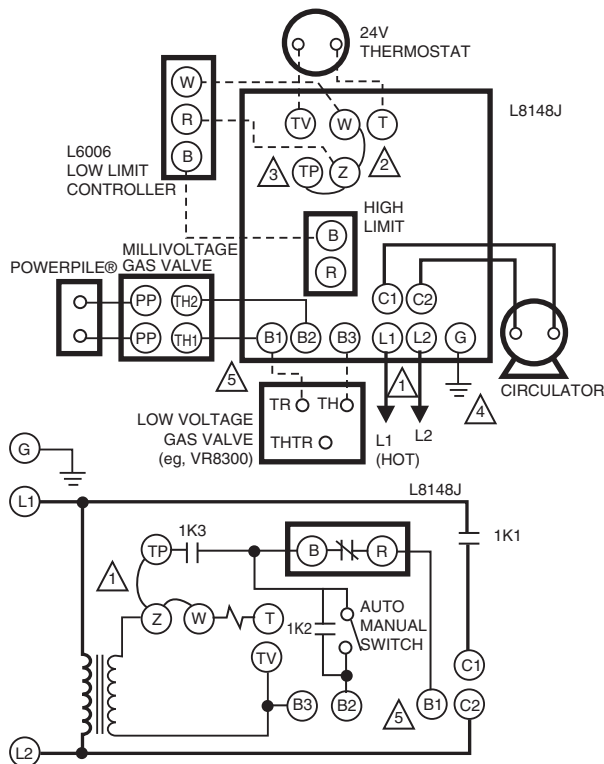
Fig. 13. Internal schematic and external connections for wiring L8148J for either low voltage or millivoltage gas valves.
