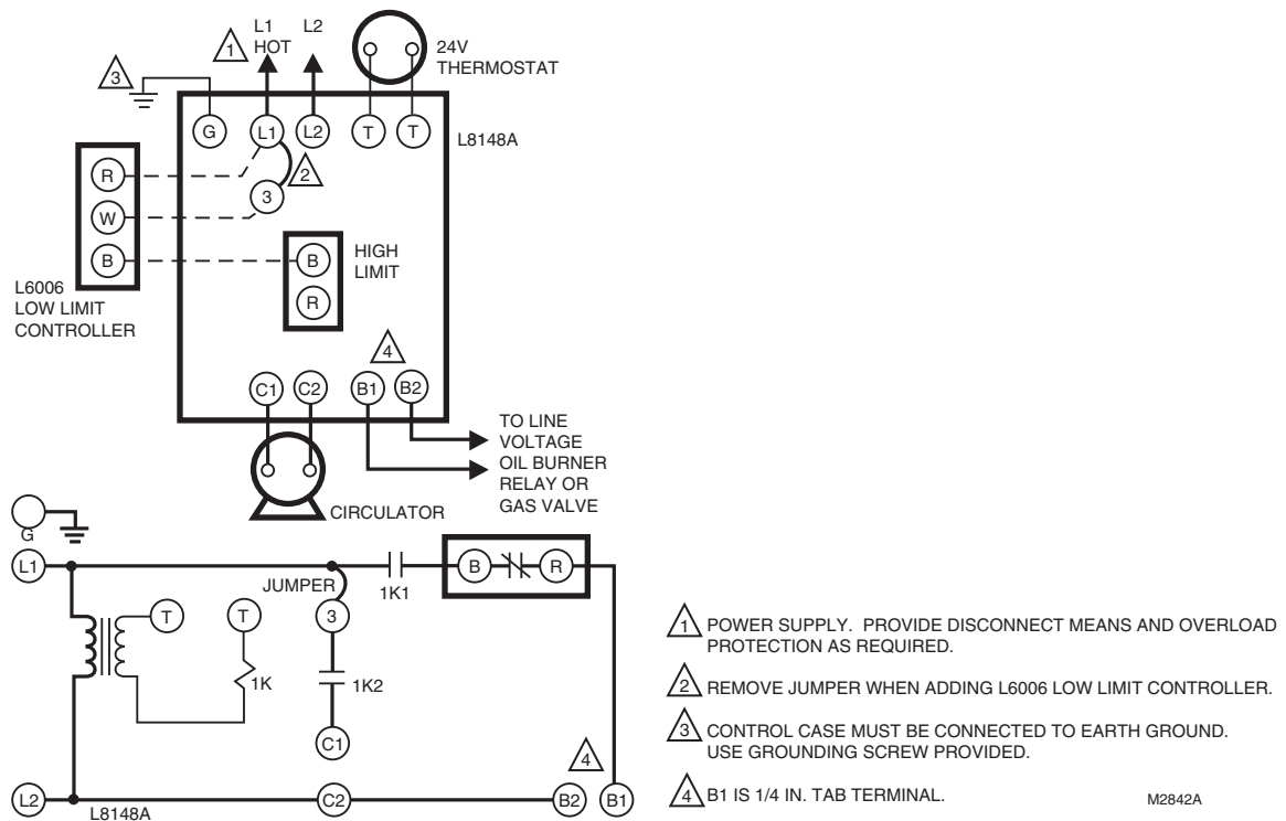
Fig. 5. External connections and internal schematic for L8148A.
