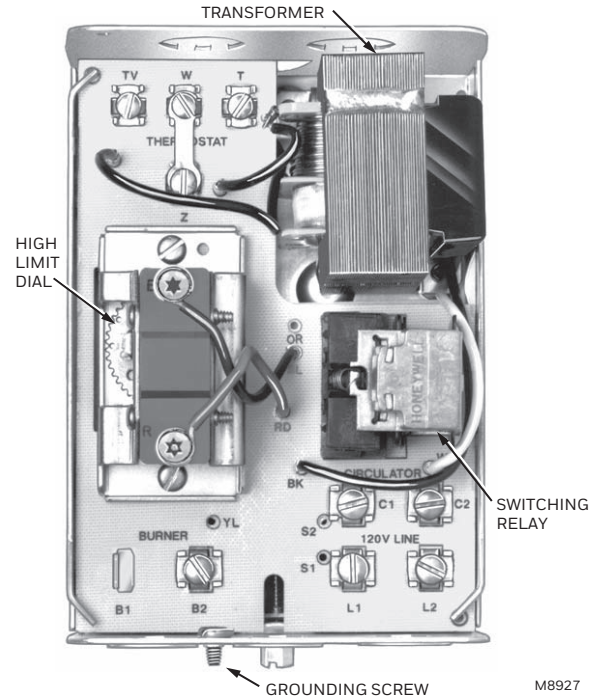
Fig. 3. Internal view of L8148E Aquastat® Relay.
