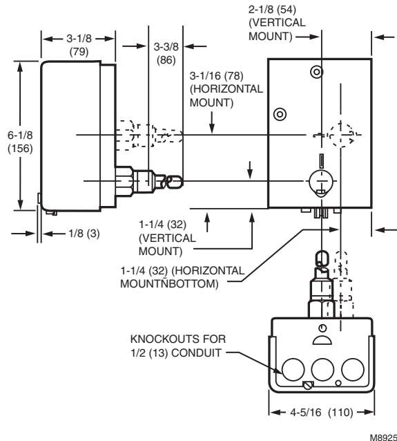
Fig. 1. L8148 dimensions in in. (mm).
