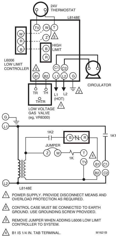
Fig. 7. External connections and internal schematic for L8148E.
