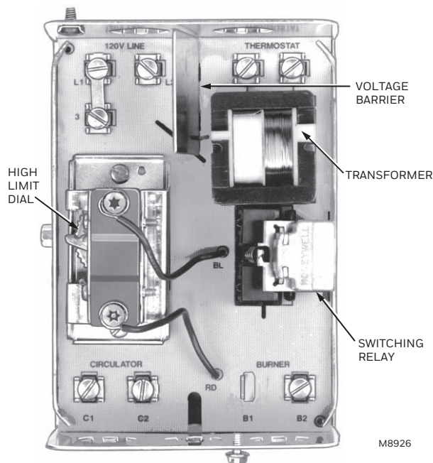
Fig. 2. Internal view of L8148A Aquastat® Relay.
