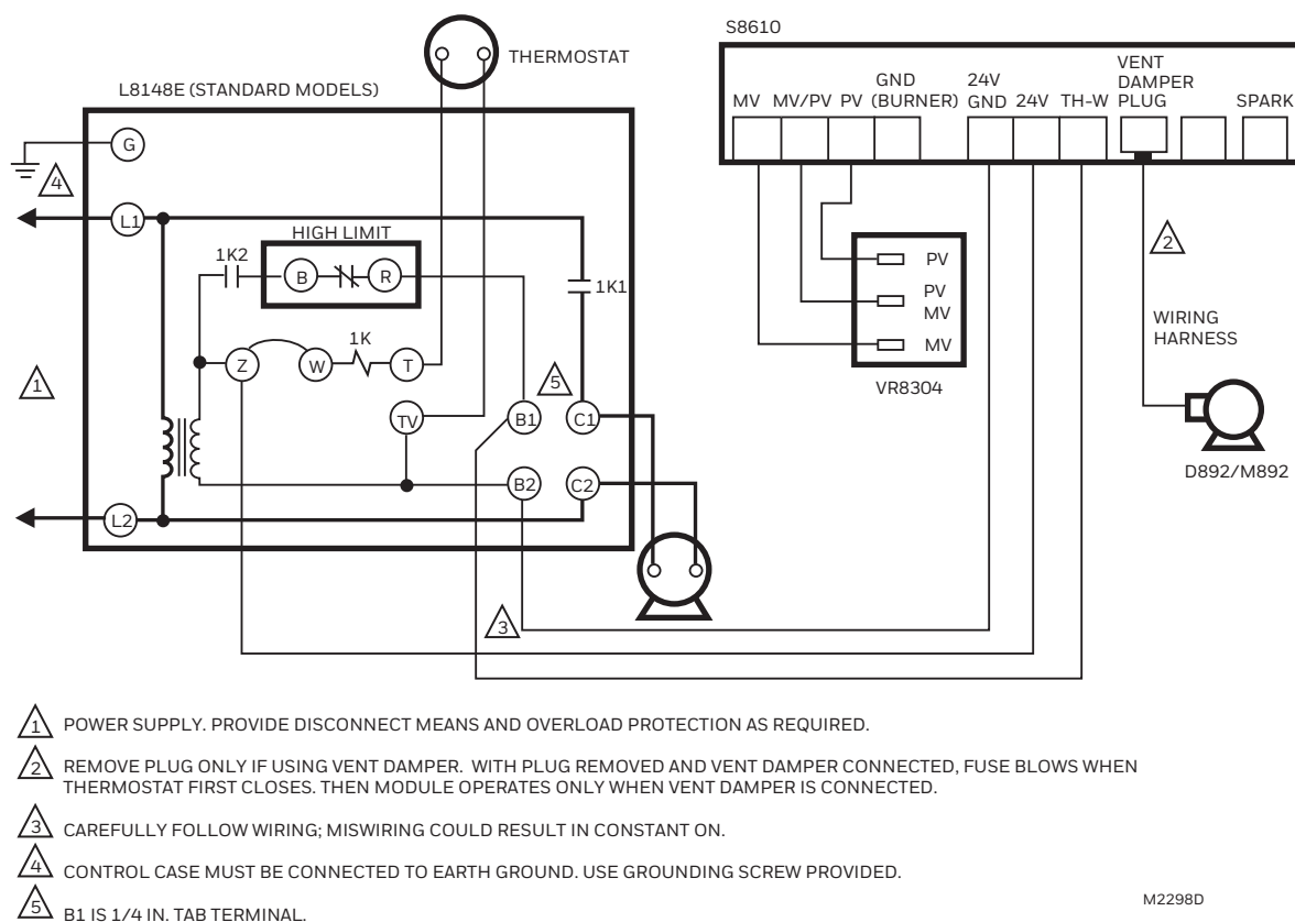
Fig. 11. Wiring L8148E with S8610A,F Intermittent Pilot Ignition Module with automatic vent damper plug and Resideo D892/M892 Vent Damper.
