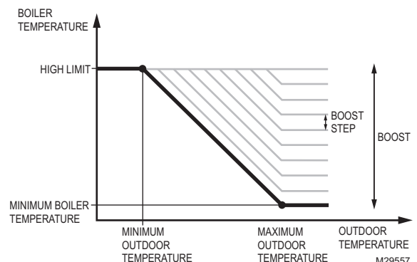
Fig. 3. Outdoor temperature setback curve with boost.
