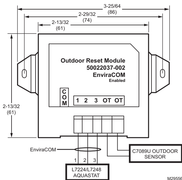
Fig. 1. 50022037-002 Outdoor Reset Module wiring diagram.
