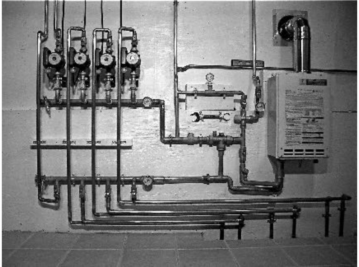
Some do-it-yourselfers create art with our installation packages. The above example uses a Takagi on-demand water heater to provide both domestic hot water and four zones of space heating
