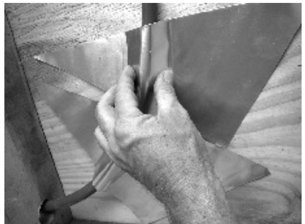
Radius plates are easily hand-formed around the bends
