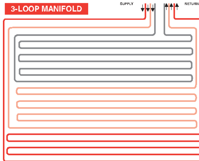
This is a commonly used layout pattern for a typical slab on grade installation. Although it's perfectly ok, and sometimes necessary, to cross one tube over another during tubing layout, notice how this simple configuration places each loop within its neighbor, starting from the outer connections of the manifold and working toward the center.
