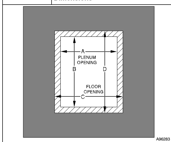
Floor and Plenum Opening Dimensions
