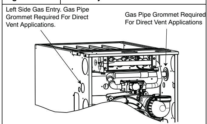
Figure 34 Gas Entry
