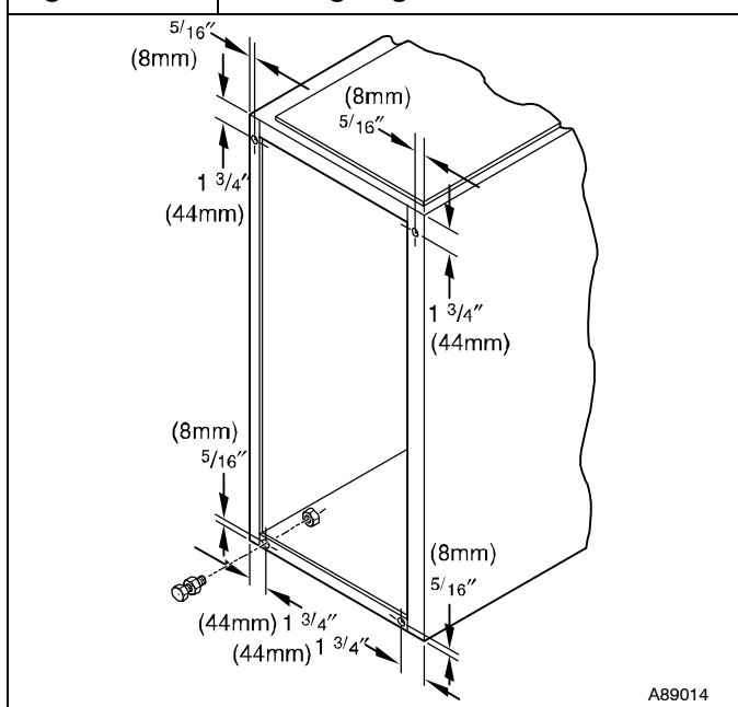
Figure 20 Leveling Legs
