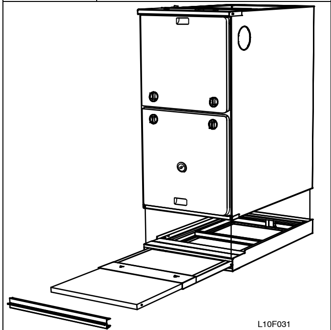
Figure 30 Accessory Bottom Filter Rack
