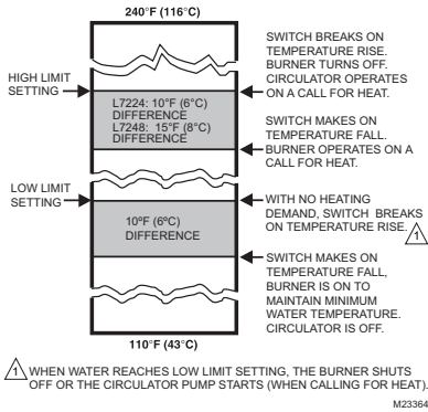
Fig. 7. Setpoints and differentials.
