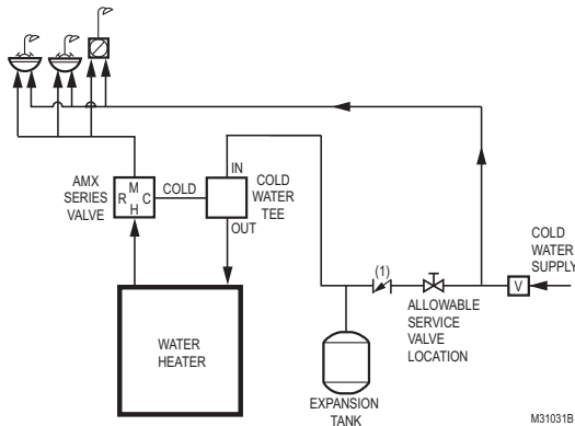
Fig. 4. ASSE 1017 compliant installation without recirculation.
