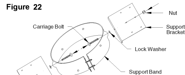
Roof Support Assembly
