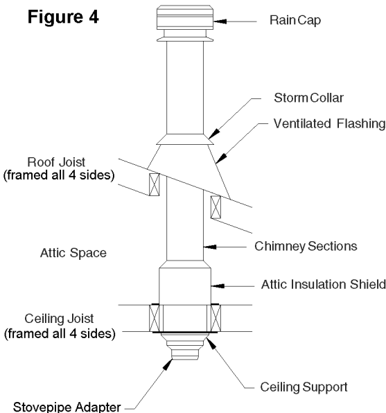
Single-Story Installation
