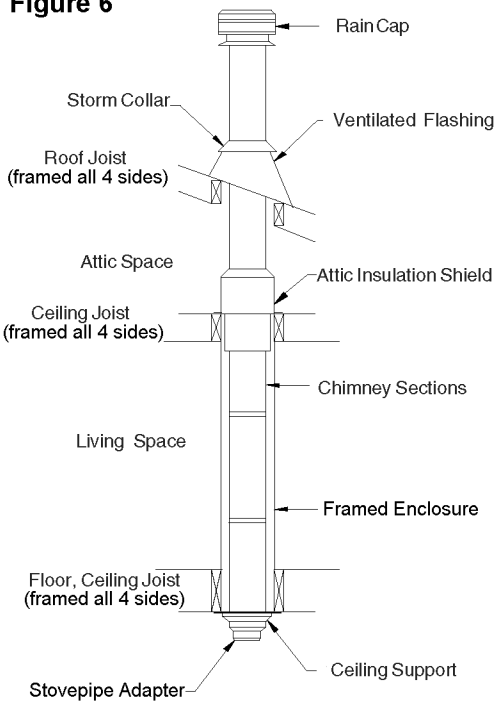
Two-Story Main Floor Installation
