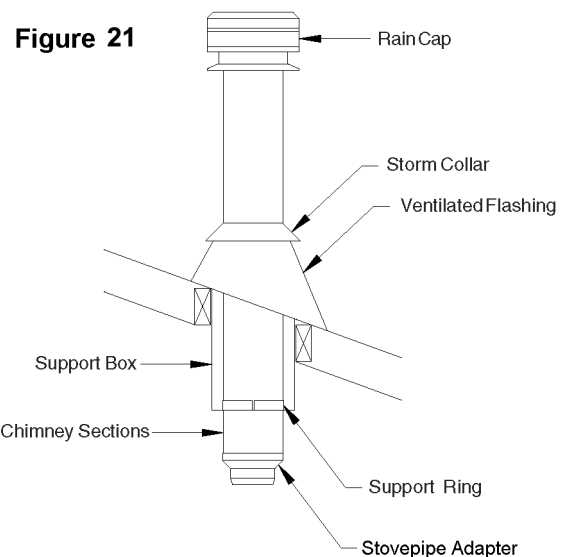
Figure 21 Cathedral Ceiling Support Installation
