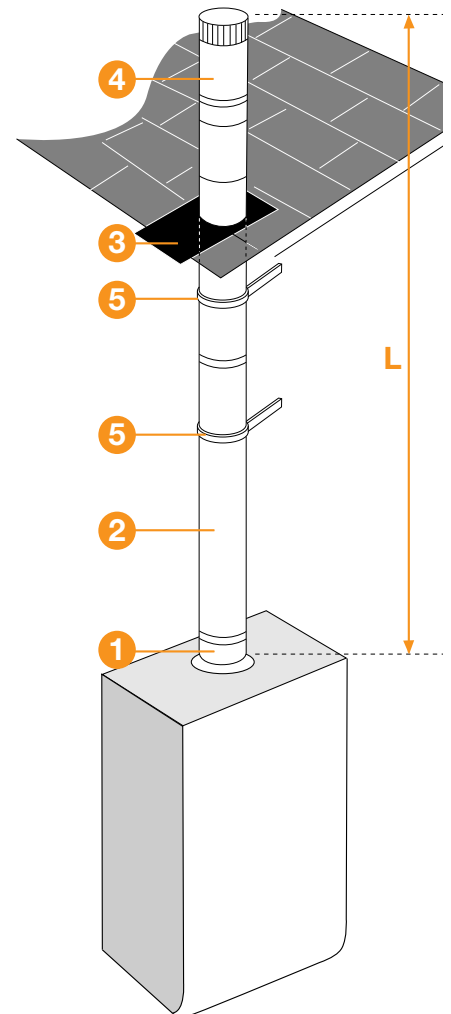
Fig 5 Maximum permissible flue length = L
