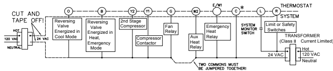
Figure 4. Typical wiring diagram for two transformer heat pump systems with NO safety circuits
