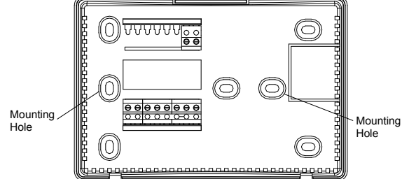
Figure 2. Thermostat base
