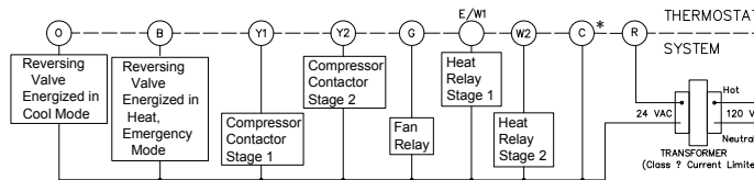
Figure 5. Typical wiring diagram for single transformer multi-stage systems
