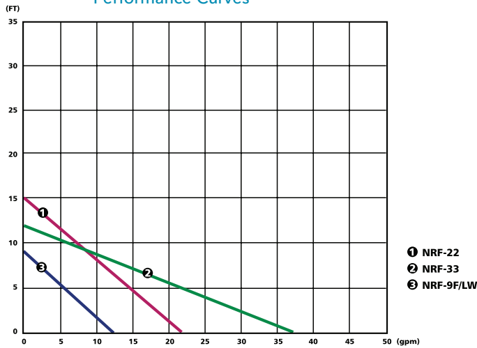
Single Speed NRF Circulator Performance Curves
