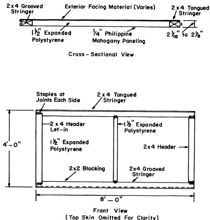
Fig. 2. Section and Elevation of Stressed-Skin Panel
