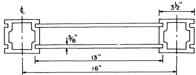
Fig. 1. Cross Section of Asbestos-Cement Panel
