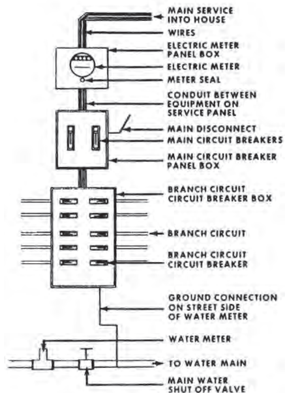
Figure 11.11. Two-wire Service [2]
