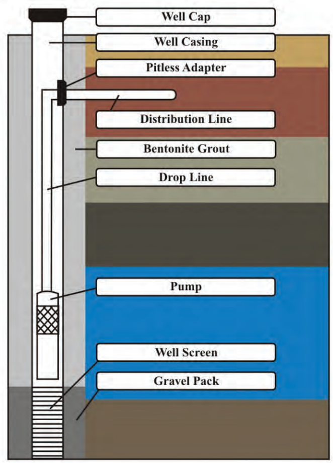
Figure 8.6. Drilled Well [4]
