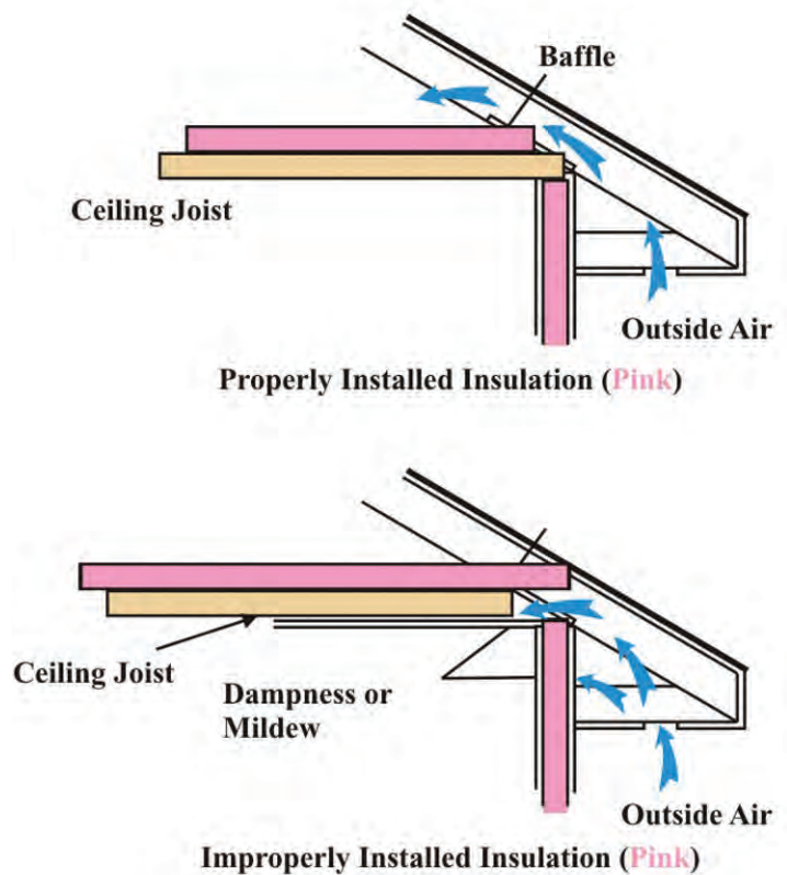
Figure 7.4. Attic ventilation
