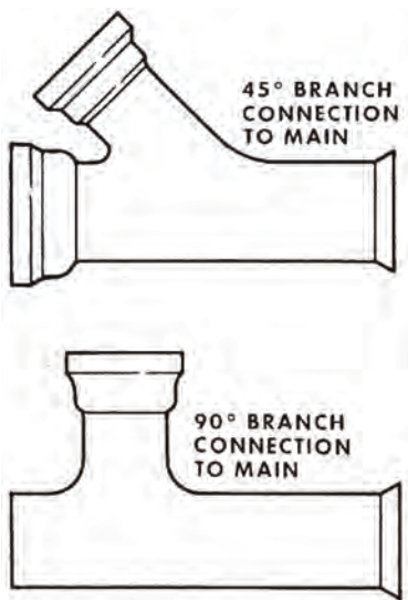
Figure 9.5. Branch Connections
