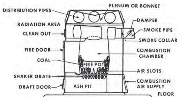
Figure 12.13. Warm-air Convection Furnace [4]
