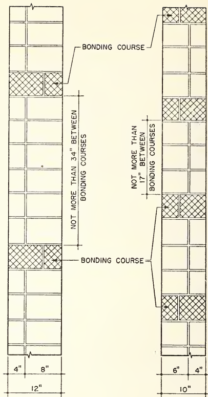
LAPPING WITH UNITS AT LEAST 3\frac{1}{2} " OVER UNITS BELOW
