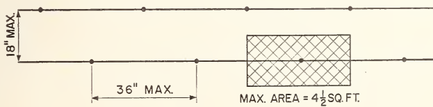
Figure 2. Spacing and staggering of metal ties.
