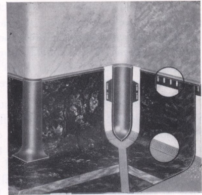
Metal inside and outside corner pieces, for linoleum flash type coving are illustrated in this cutaway view. The wax fillet strip supports the material at the point of the curvature. Adhesive and the binding strip hold it in place.
