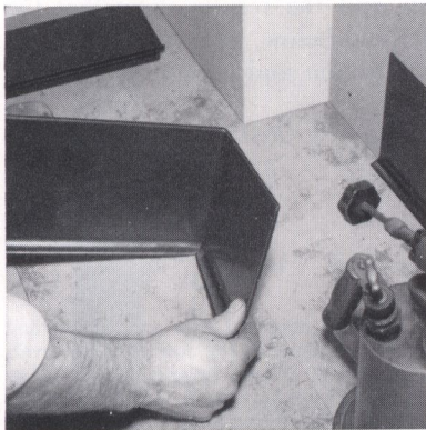
Inside corners are formed by heating and cutting a notch from the flange and fitting the base to the corner. Outside corners can also be fitted and formed in a single piece without seams by heating base and forming it to corner.
