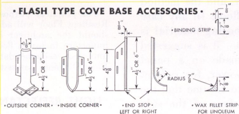
Inside corners are formed by heating and cutting a notch from the flange and fitting the base to the corner. Outside corners can also be fitted and formed in a single piece without seams by heating base and forming it to corner.
