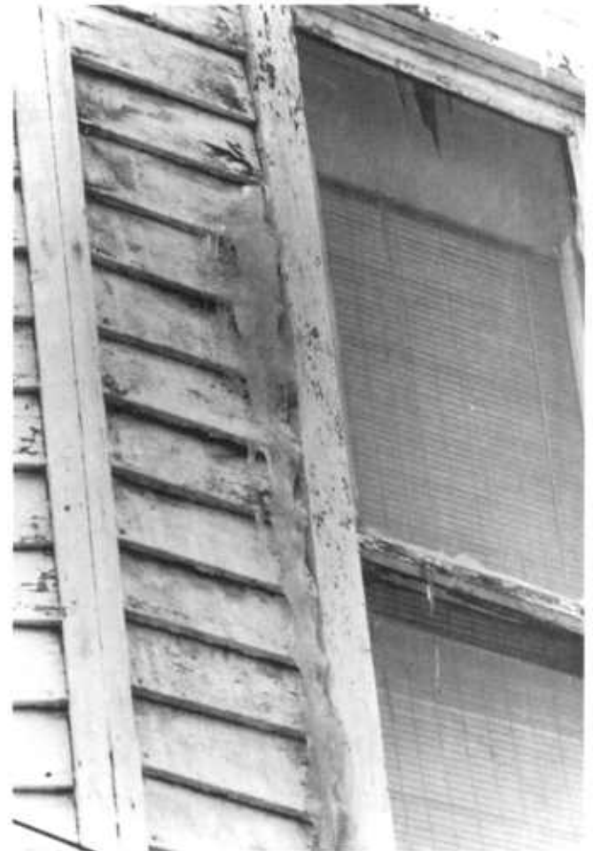
Figure 7 —Cold weather condensation on a house without a vapor barrier on interior walls. Paint blistering, peeling, and wood decay are likely.
