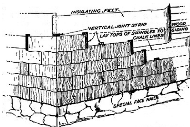
Figure 4. Asbestos-Cement siding installation specifications (McCawley, 1940).
