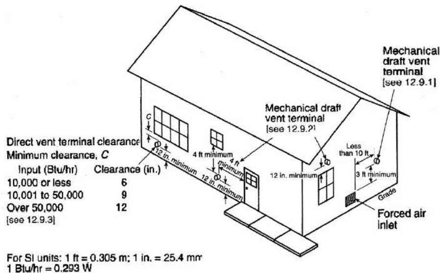
Figure 2. Combustion air and vent terminal locations (Source: 2012 National Fuel Gas Code, Copyright American Gas Association. Used with Permission.)
