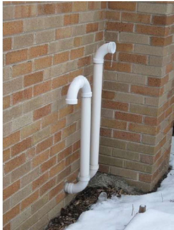
Figure 12. Vent termination above the snow line
