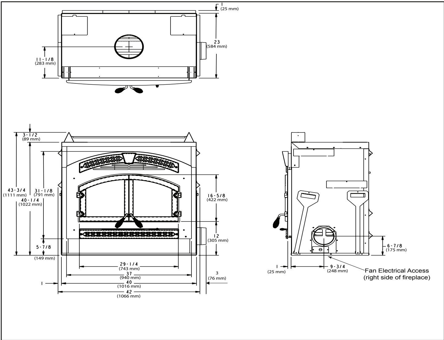
Figure 3.1 Fireplace Dimensions
