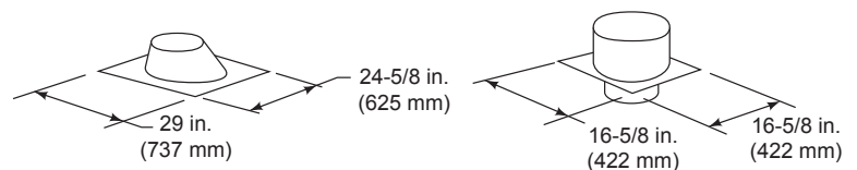
MH841 Manufactured Home Thimble Extension
