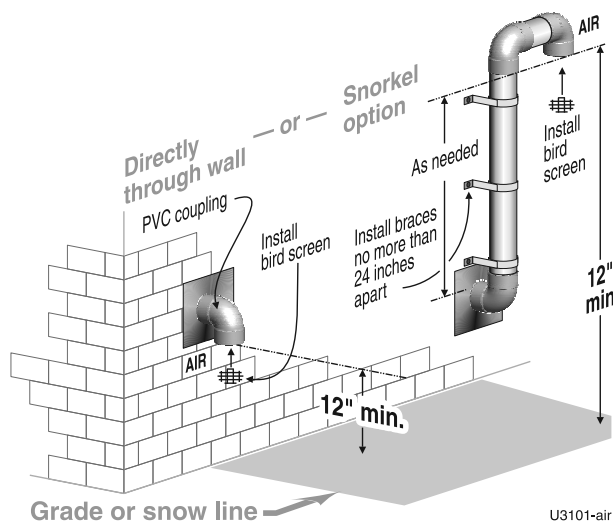
Figure 21 Sidewall air inlet (termination) for direct vent: vertical vent / sidewall air
