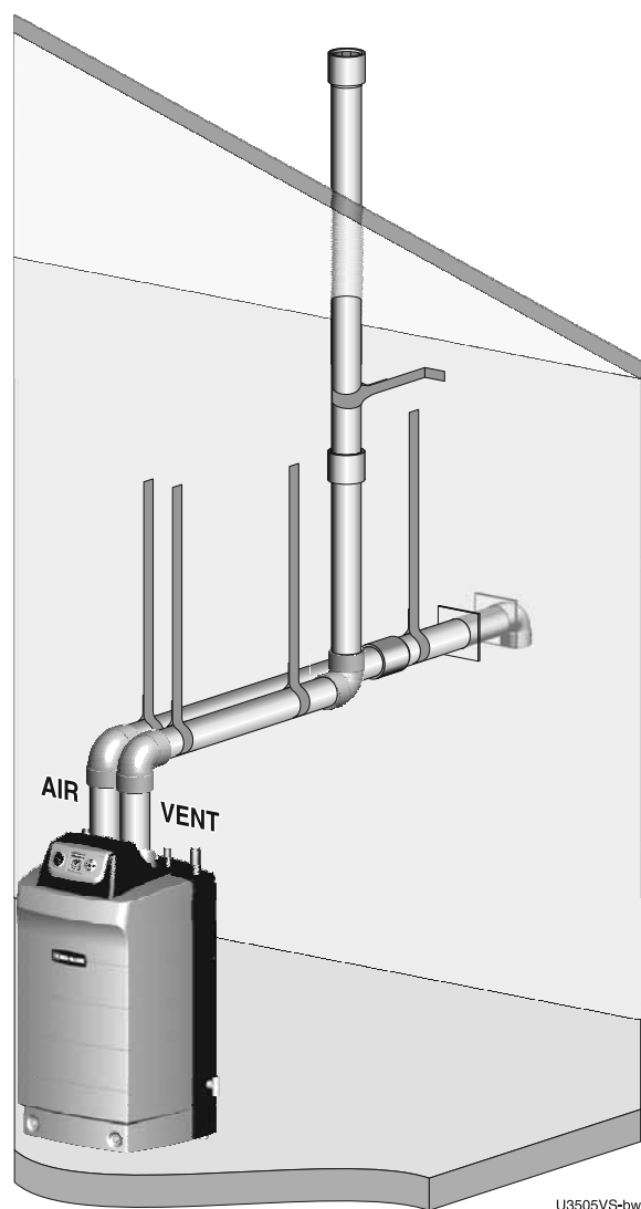
Figure 19 Direct vent: Vertical vent / sidewall air
