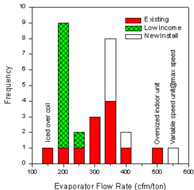
Figure 2 Histogram of evaporator airflow rates
