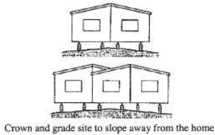
Figure to § 3285.203 - Grading and drainage.
