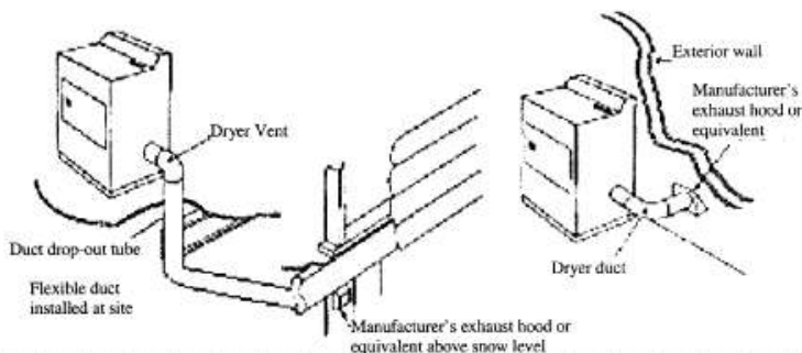
Figure A to § 3285.503 Dryer Exhaust System.
