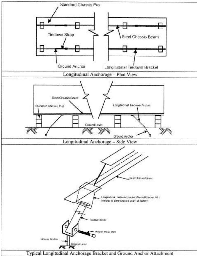
Figure C to § 3285.402 Longitudinal Anchoring
