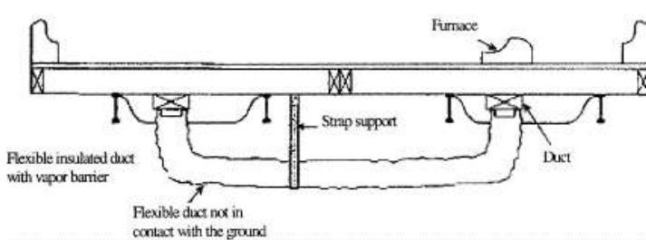
Figure B to §3285.606 Crossover Duct Installation with One Connecting Duct.
