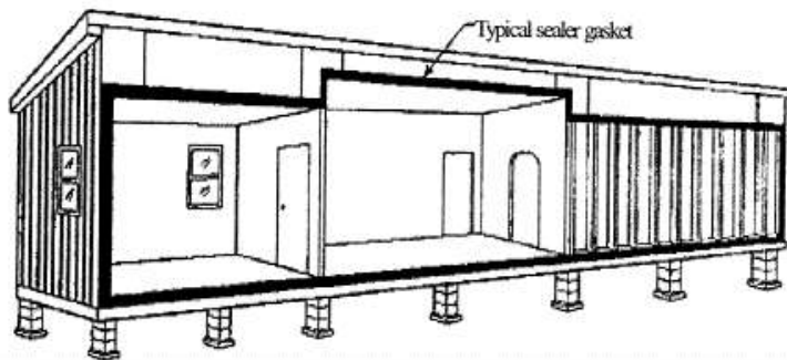
Figure B to § 3285.801 Mate-Line Gasket.
