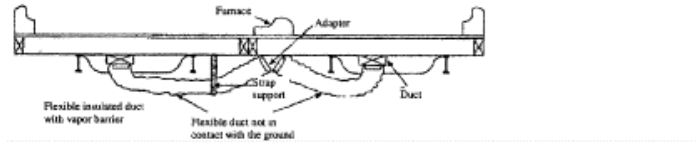
Figure A to §3285.606 – Crossover Duct Installation with Two Connecting Ducts.
