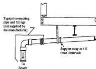
Figure A to § 3285.904 – Connection to Site Sewer.
