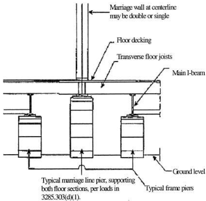
Figure C to § 3285.310 Typical Mate-Line Column and Piers.
