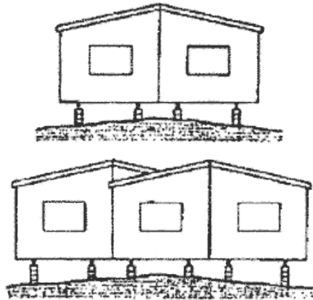
Figure to § 3285.203 - Grading and drainage.
