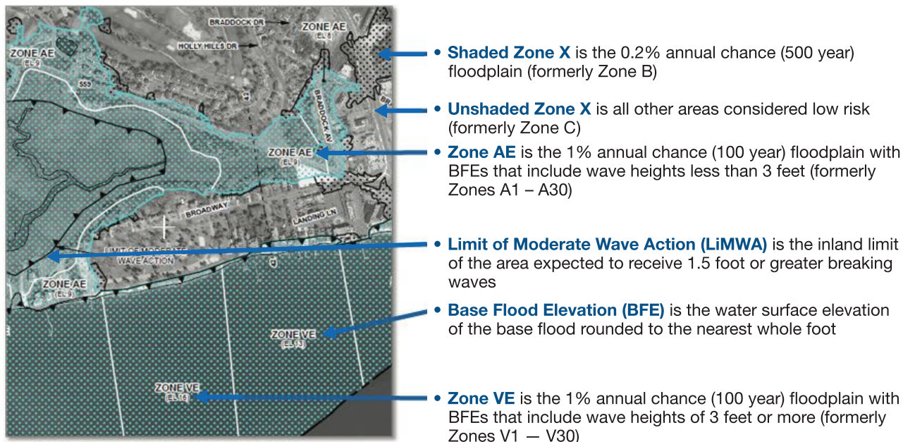
Figure 1-3. Conceptual FIRM showing representative coastal flood zones.
